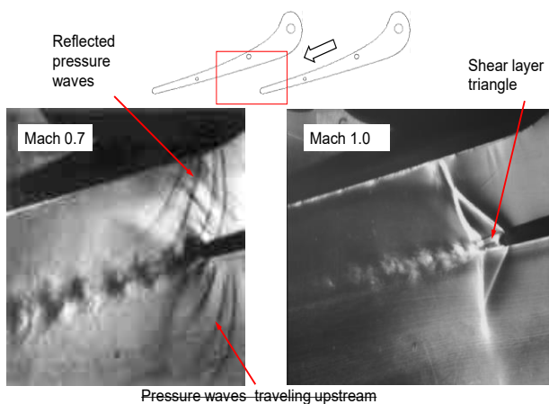
Figure 4 Subsonic and Transonic Schlierens
