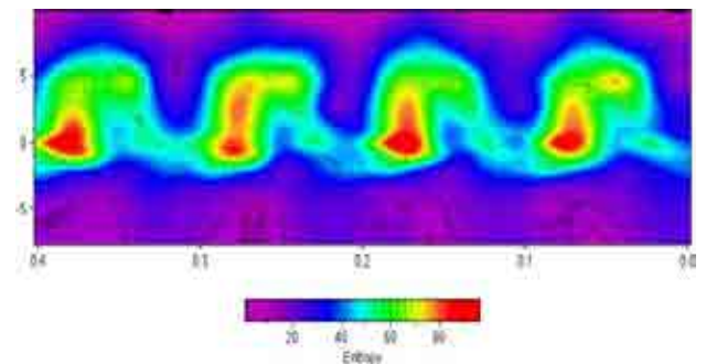
Figure 3 Time-resolved entropy contours downstream of the cascade trailing edge.
