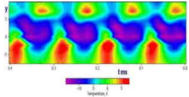
Figure 2 Time-resolved temperature contours
