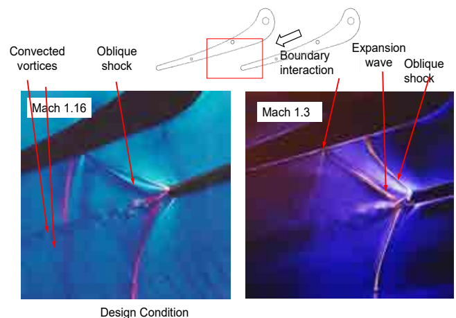
Figure 5 Transonic and Supersonic Schlierens
