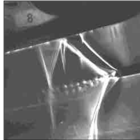
Figure 6 Shedding of Couples at Ma = 1.07
