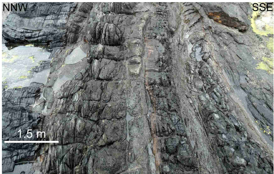
984 Figure S-2. Multiple injection, sub-vertical dyke striking ENE-WSW, indicating preferential 985 NNW-SSE opening.
