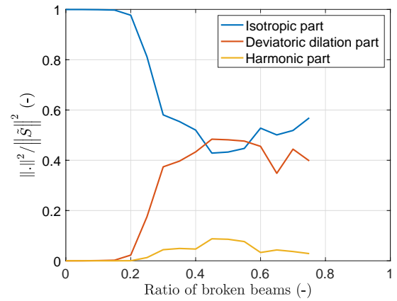
Figure 16: Willam loading: Evolution of the relative parts of the effective compliance tensor with the ratio of broken beams.
