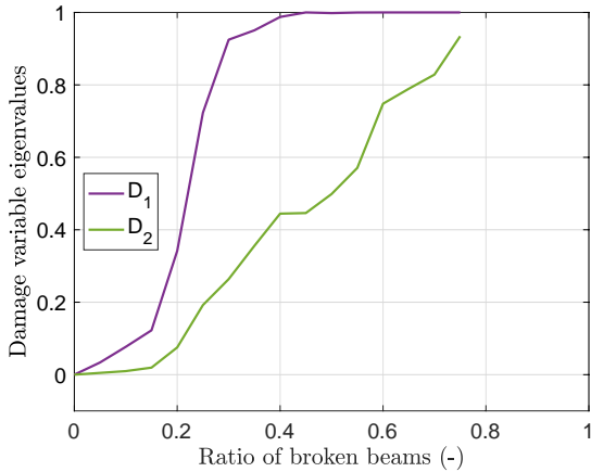
Figure 32: Willam loading: Evolution of the eigenvalues of the damage tensor \mathbf{D} with the ratio of broken beams.
