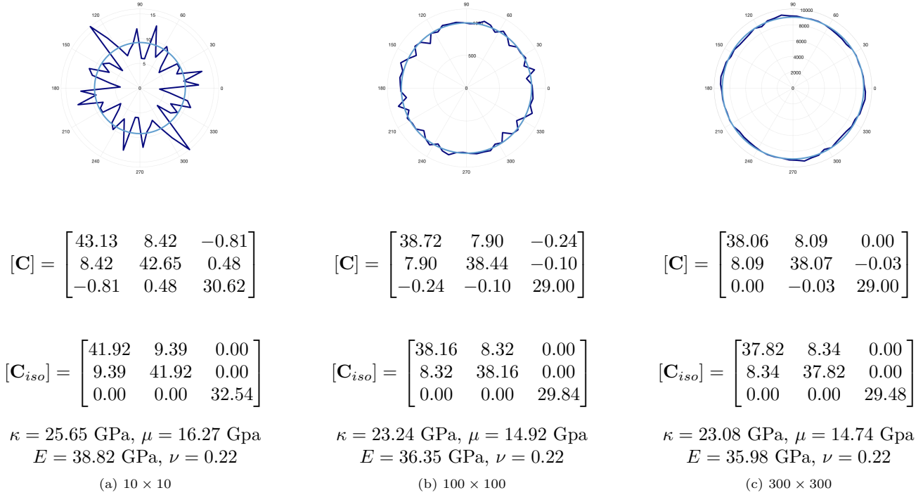
Figure 3: Polar histograms of the beams orientation for different mesh densities, elasticity tensors and associated isotropic tensors (in GPa, Kelvin representation).
