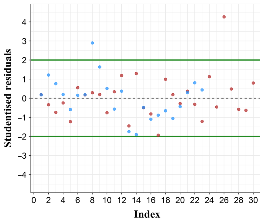
Fig. 2. Studentized residuals associated with each regression. Red dots represent studentized residuals associated with DNA standard curve ( n = 30 ). Blue dots represent studentized residuals associated with RNA standard curve ( n = 24 ).
