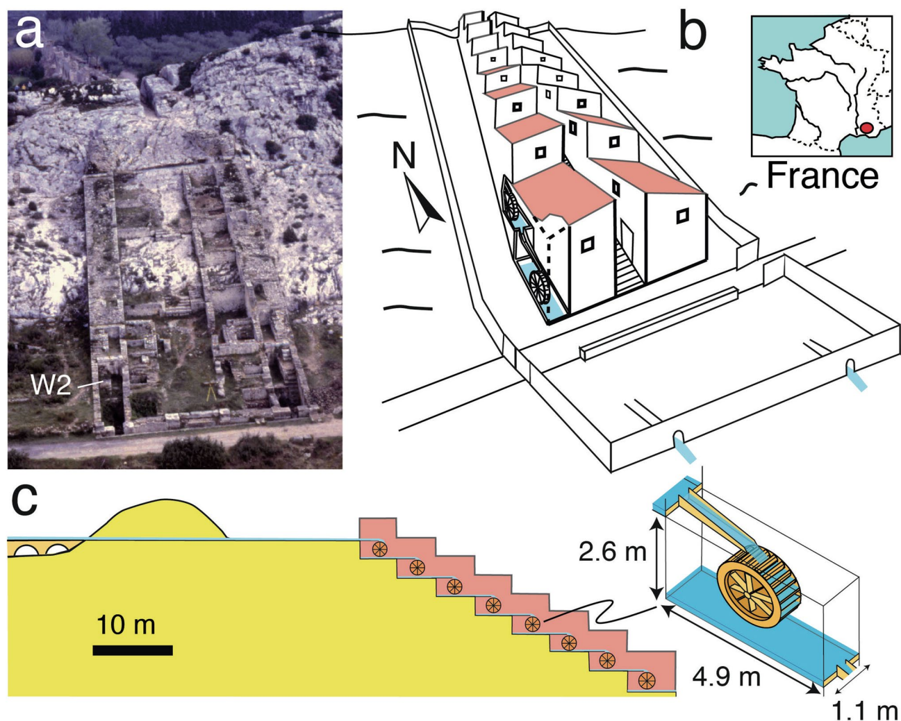
Figure 1. The Barbegal watermill complex, built in the second century CE in Southern France. (a) Ruins of the complex photographed in 1996, seen from the south. The aqueduct feeding the mills entered from the north through a rock cut seen at the top. W2 is the mill basin where carbonate was found in the axle window. The elbow flume was probably located in this basin, or the one below. (b) Reconstruction of the two parallel trains of eight mills (of which two are shown) that were built on a natural slope, with central buildings. Inset shows the location in France. (c) N–S cross-section of the mill complex along one train of millwheels, drawn to scale, with a close-up drawing of one mill.
