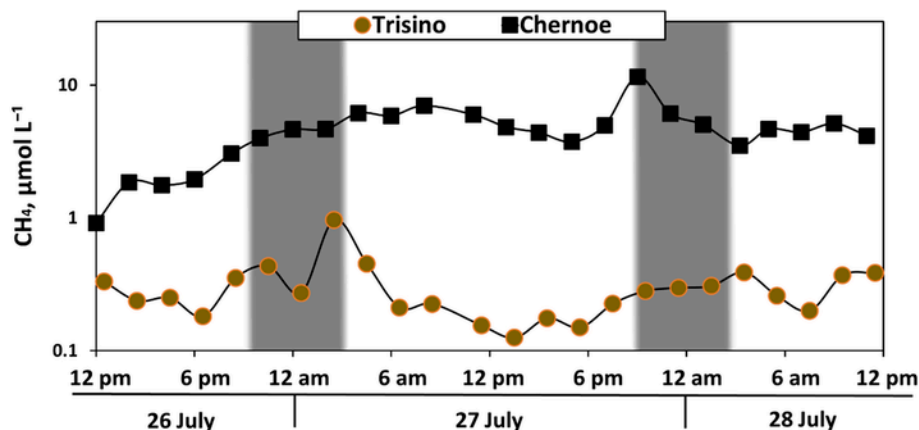
Fig. 3. Diurnal pattern concentration of dissolved \text{CH}_4 measured in the two lakes of Western Siberia. The uncertainties of \text{CH}_4 concentration are within the symbols size. They stem from 2 to 3 individual measurements in various part of the lake at each time of the day.
