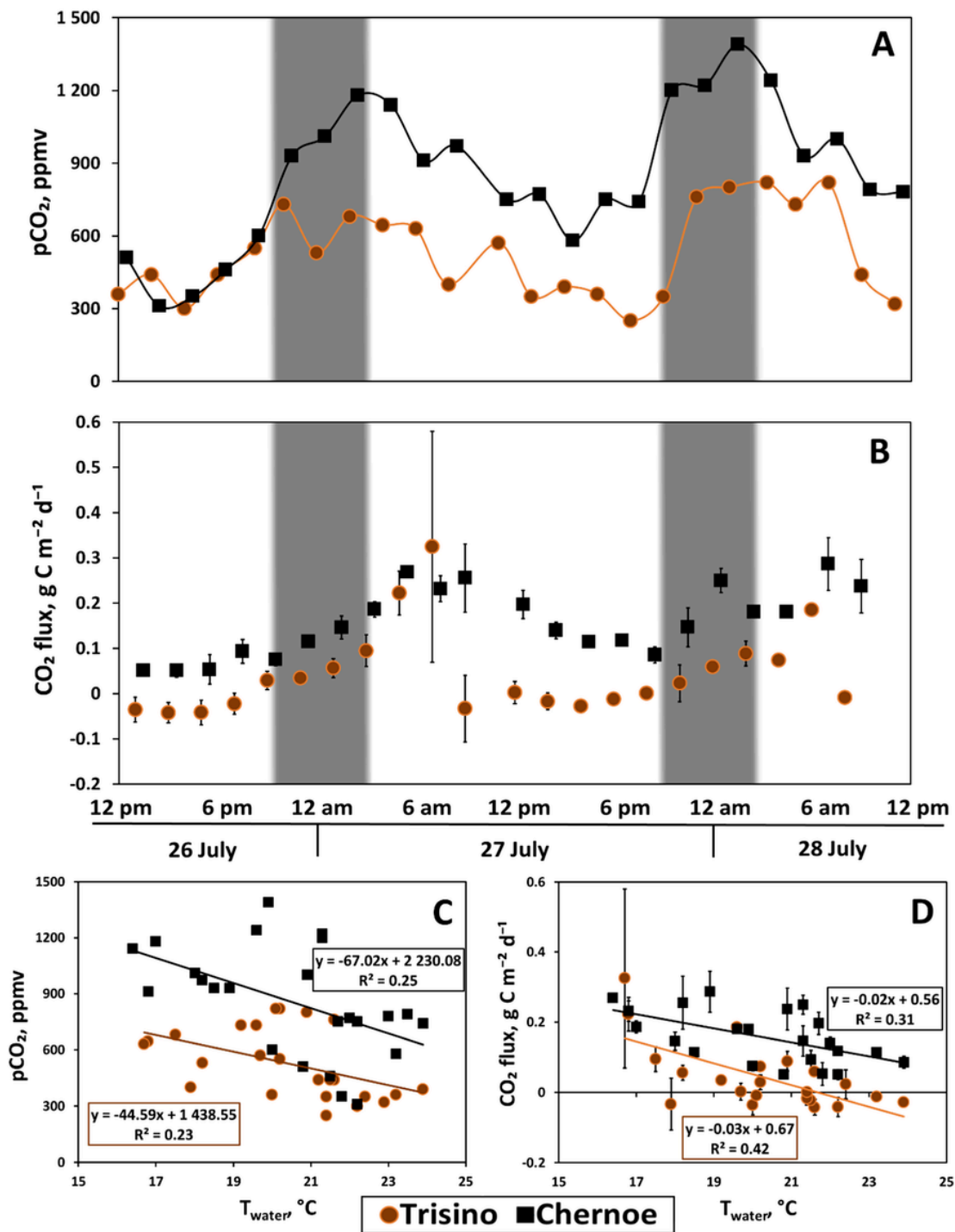
Fig. 2. Diurnal pattern of pCO 2 (A) and CO 2 flux (FCO 2 ) (B) measured in the two lakes of Western Siberia. The negative correlations between pCO 2 and water temperature (C) and FCO 2 and water temperature (D) are significant at p < 0.01. The error bars represent the s.d. of six (Trisino) and four (Chernoe) chamber measurements across the lakes.
