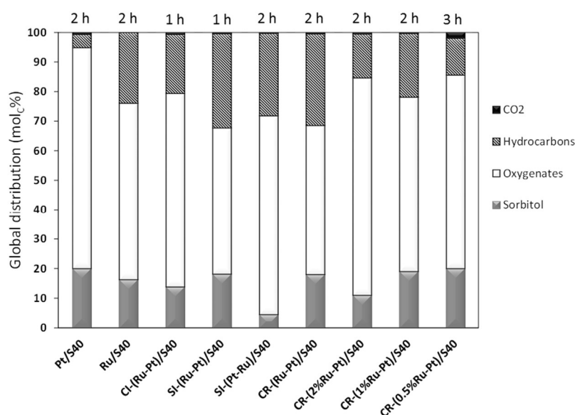
Figure 6. Carbon global distribution obtained at 80–96% sorbitol conversion for the Ru-Pt/S40 bimetallic catalysts prepared by co-impregnation (CI), successive impregnations (SI) and catalytic reduction deposition (CR), as well as for Pt and Ru monometallic catalysts.
