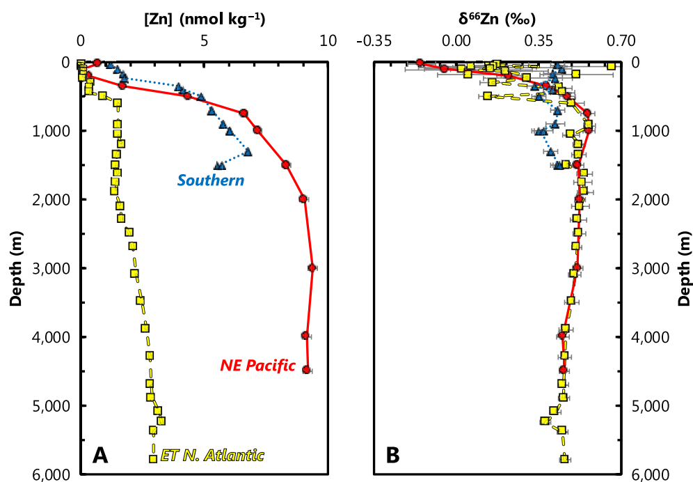
Figure 9. Representative profiles of dissolved Zn concentrations ( [Zn] ); (a) and Zn isotopic compositions ( \delta^{66}\text{Zn} ); (b). Data from the Eastern Tropical North Atlantic (squares, dashed line; Conway & John, 2014b), Northeast Pacific (circles, solid line; Conway & John, 2015a) and Southern Oceans (triangles, dotted line; R. M. Wang et al., 2019). Station locations as per Figure 1. This comparison illustrates that despite possessing distinct dissolved concentration profiles, the isotopic behavior of Zn is similar between basins.
