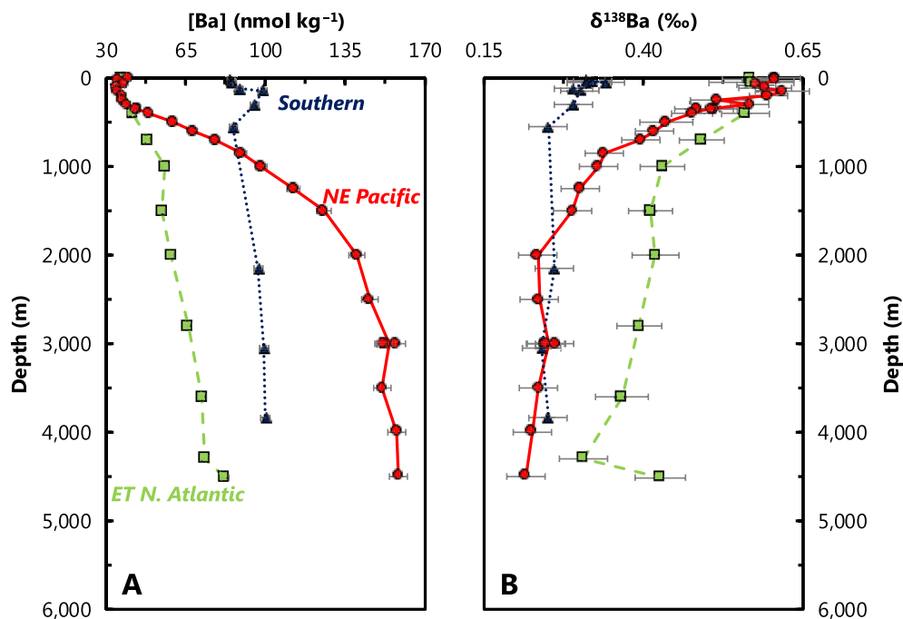
Figure 22. Representative profiles of dissolved Ba concentrations ( [Ba] ); (a) and Ba isotope compositions ( \delta^{138}\text{Ba} ); (b). Data from the Eastern Tropical North Atlantic (squares, dashed line; Bates et al., 2017), Northeast Pacific (circles, solid line; Geyman et al., 2019), and Southern Oceans (triangles, dotted lines; Hsieh & Henderson, 2017). Station locations as per Figure 1. This comparison illustrates that the oceanographic processes leading to distinct dissolved concentration profiles render significant changes in dissolved \delta^{138}\text{Ba} between basins.
