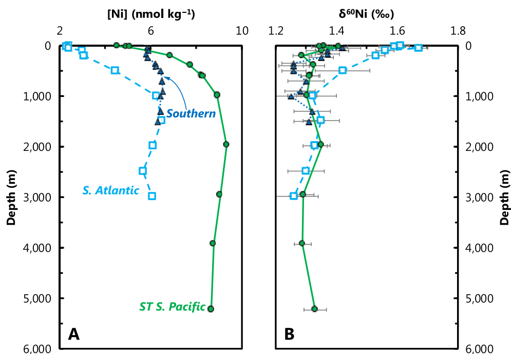
Figure 24. Representative profiles of dissolved Ni concentrations ( [Ni] ); (a) and Ni isotopic compositions ( \delta^{60}\text{Ni} ); (b). Data from the South Atlantic (squares, dashed line; Archer et al., 2020), Southern (triangles, dotted line; R. M. Wang et al., 2019), and Subtropical South Pacific Oceans (circles, solid line; Takano et al., 2017). Station locations as per Figure 1. This comparison illustrates that the oceanographic processes leading to distinct dissolved concentration profiles render only small changes in dissolved \delta^{60}\text{Ni} between basins.
