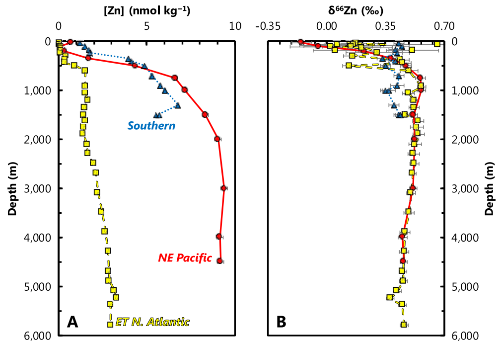
Figure 9. Representative profiles of dissolved Zn concentrations ( [Zn] ); (a) and Zn isotopic compositions ( \delta^{66}\text{Zn} ); (b). Data from the Eastern Tropical North Atlantic (squares, dashed line; Conway & John, 2014b), Northeast Pacific (circles, solid line; Conway & John, 2015a) and Southern Oceans (triangles, dotted line; R. M. Wang et al., 2019). Station locations as per Figure 1. This comparison illustrates that despite possessing distinct dissolved concentration profiles, the isotopic behavior of Zn is similar between basins.
