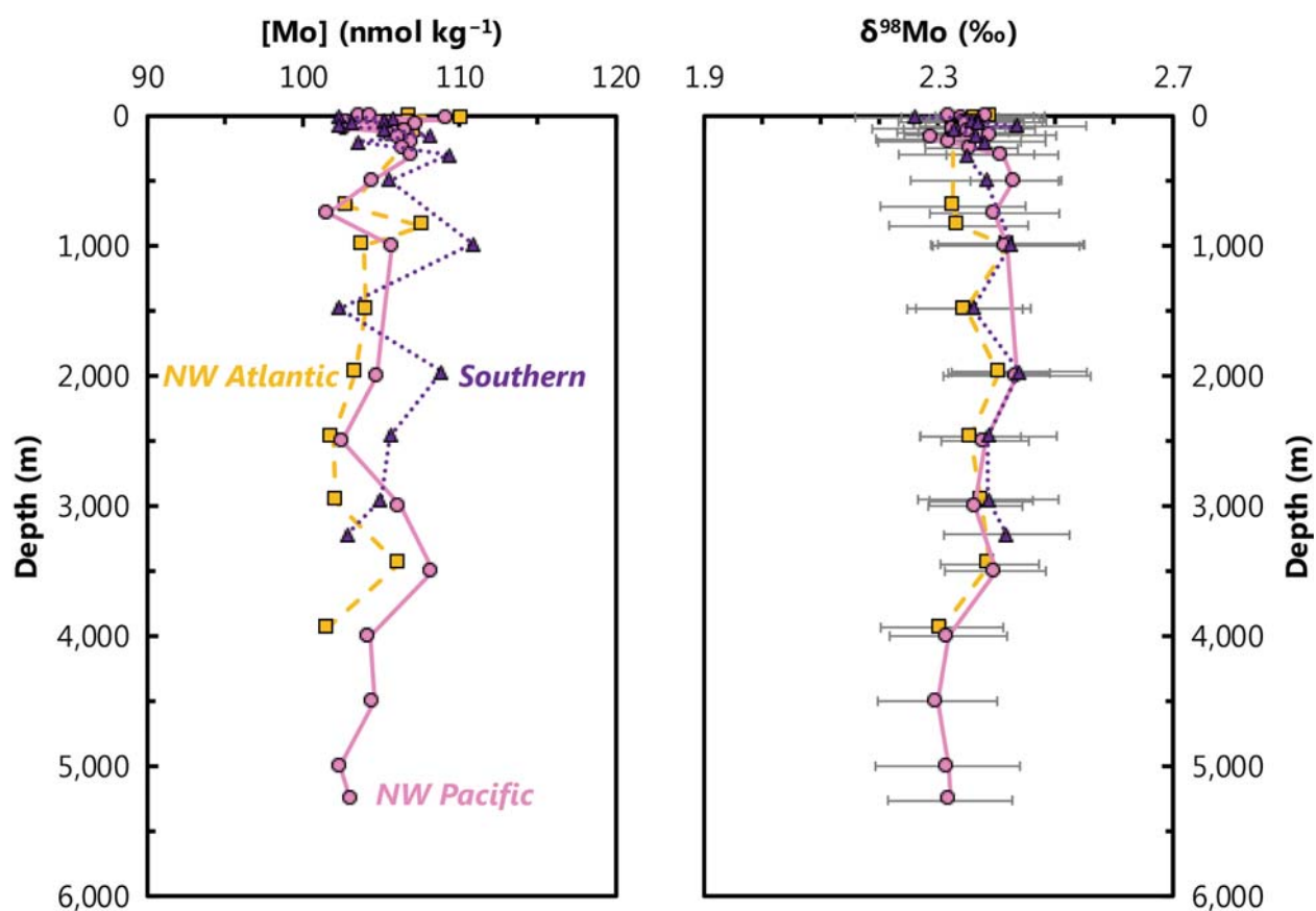
1269 Figure 16 | Representative profiles of dissolved Mo concentrations ([Mo]) and Mo-isotopic compositions 1270 ( \delta^{98}\text{Mo} ) in the Northwest Atlantic (squares, dashed line), Southern (triangles, dotted line), and Northwest 1271 Pacific (circles, solid line) Oceans. This comparison illustrates that the dissolved behavior of Mo is essentially 1272 invariant throughout the global oceans. 1273
