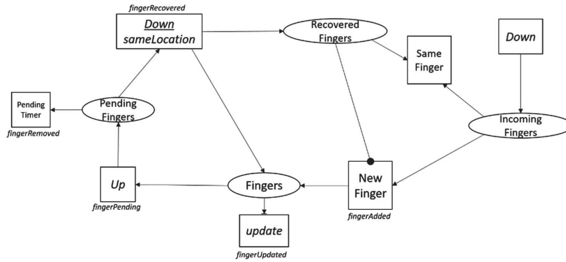
Fig. 5. Abstract behavioral model of the finger manager
