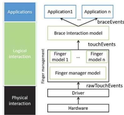
Fig. 3. High-level software architecture of brace interaction
