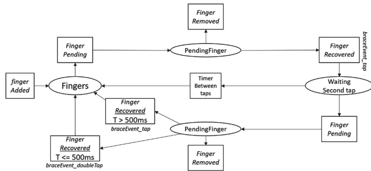
Fig. 7. Abstract model of Brace Touch interaction behavior
