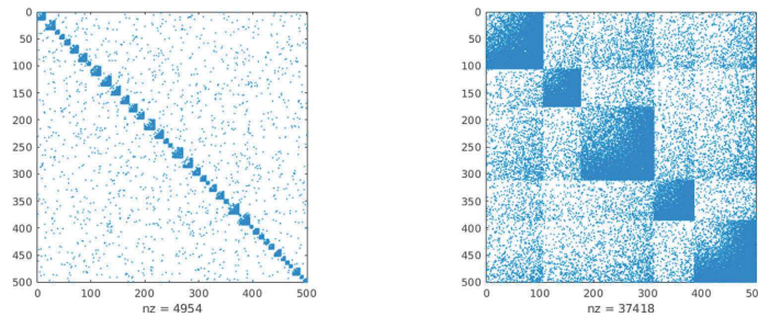
Fig. 6. Adjacency matrices of two networks
