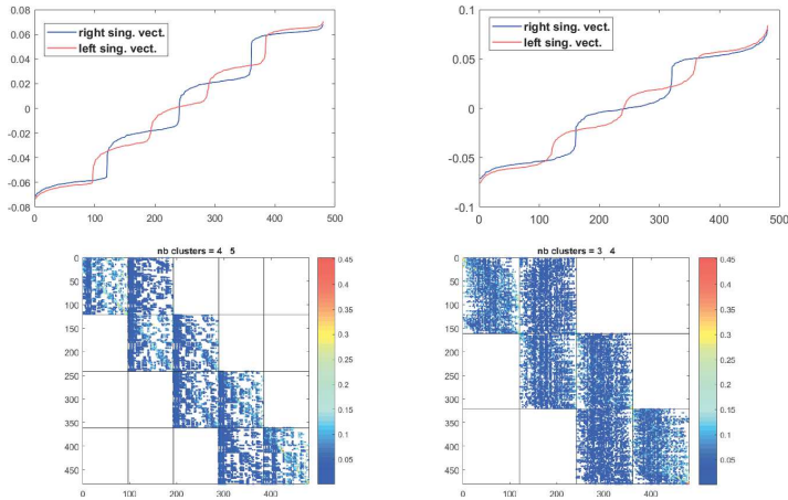
Fig. 3. Cluster identification using different singular vectors
