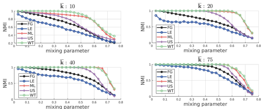
Fig. 5. Curves of NMI for FG, LE, ML, WT, US
