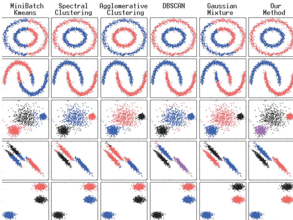
Fig. 10. Comparison between clustering algorithms
