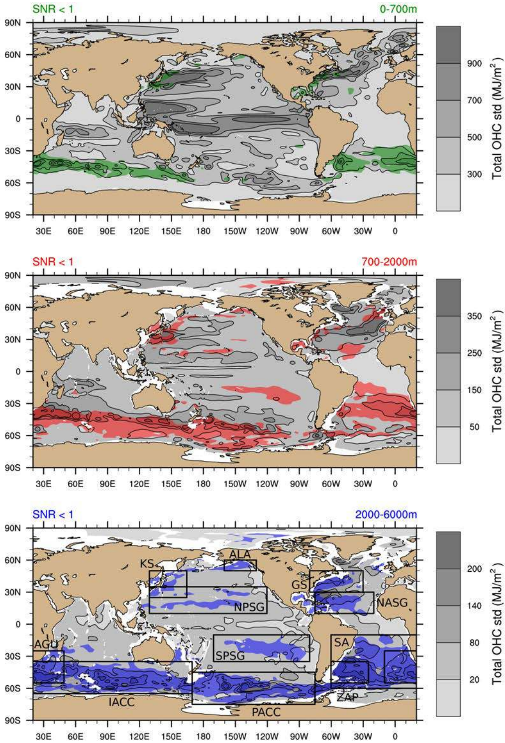
Figure 1. Total (forced+chaotic) interannual-to-decadal OHC standard deviation (std, gray shading) at scales larger than 10^\circ \times 10^\circ , shown in layers 0-700m (top), 700-2000m (middle) and 2000-6000m (bottom). Color shading indicates regions where the chaotic std exceeds the forced std. Figure 2 is focused on the OHC integrated horizontally over the regions shown in the bottom panel.
