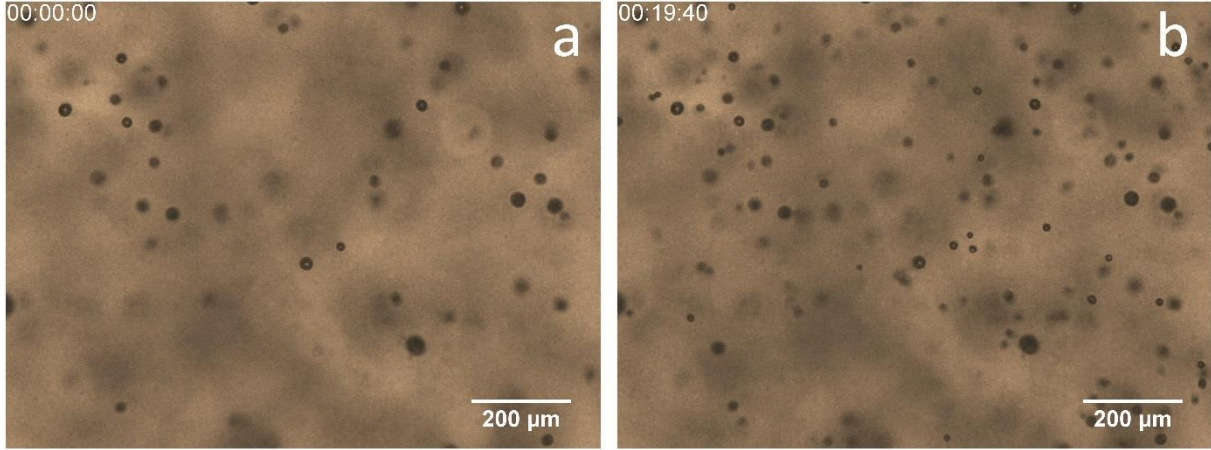
Figure 4 – Optical microscopy images of the same area in the sample D10-5 before (a) and after (b) increasing of the drying temperature from 60°C to 110°C.
