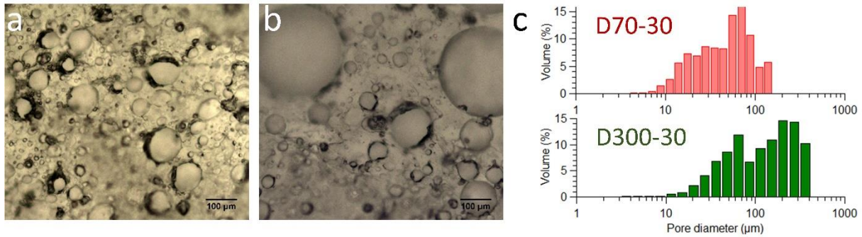
Figure 5 – Optical microscopy images of a cross-section of D70-30 (a) and D300-30 (b) samples and the corresponding volume-weighted diameter distributions (c).
