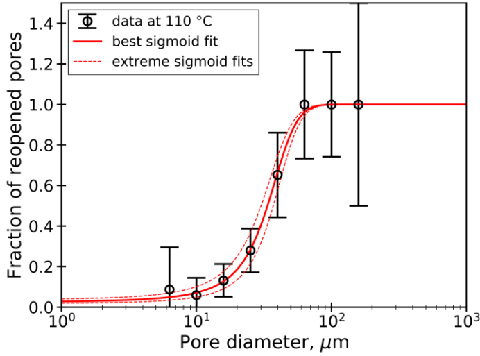
Figure 7 – Fraction of pores in sample D200-5 that reopened after drying at 110°C. The data are obtained by adding results on 4 specimens. The parameters of the fitted sigmoidal function are d_{char} = 33.6 \pm 3.5 \mu\text{m} and p = 4.0 \mu\text{m} . The error bars are obtained as 1/\sqrt{N_i} , where N_i are the numbers of pores of diameter d_i filled with water. The error on the fitted value of d_{char} is estimated by finding out the extreme values of d_{char} that make it still possible for the fitted sigmoid to remain in the experimental uncertainty.
