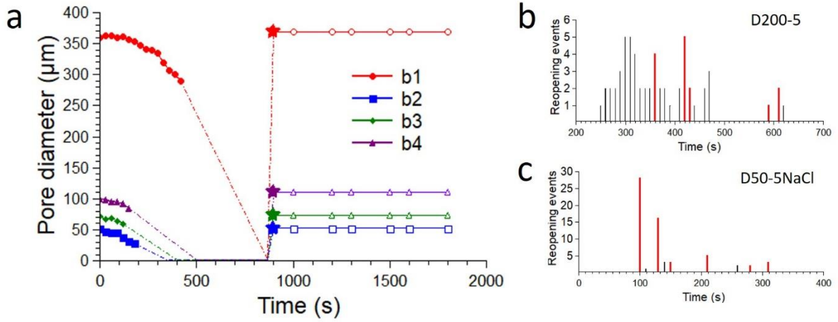
Figure 10 – a) Evolution of the pore diameter before (filled symbols) and after cavitation (open symbols) for the pores from cluster “b” on Figure 8. The points represent the data obtained when the pores had a well-defined ellipsoidal shape and were located close to the focal plane of the microscope. The supposed evolution of pore diameters after creasing instability or after eventual displacement out of the focus are represented by dashed lines to guide the eye. The moments at which reopening occurs are indicated with the star symbol. b-c) Number of cavitation events as a function of drying time at 110°C for samples D200-5 (b) and D50-5NaCl (c). The red bars correspond to reopening events of at least one pore with diameter > 50 μm.
