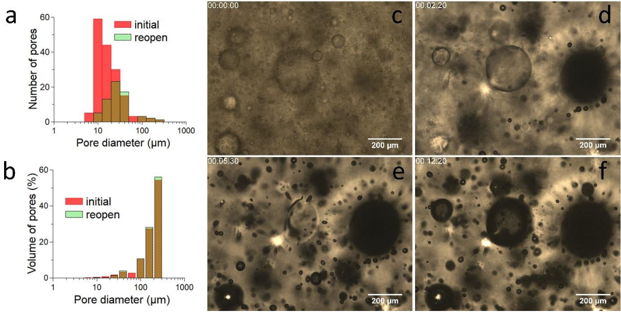
Figure 2 – a) and b) Distributions of pore diameters in the D200-5 sample obtained for initial, water-filled pores (red) and pores reopened via cavitation (semi-transparent green); c-f) optical microscopy images of the D200-5 sample during drying at 110°C. The overlap of the pore diameter distributions between water-filled and reopened pores appears as brown.
