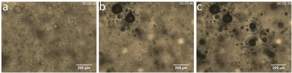
Figure 9 – Optical microscopy images showing the reopening pore clusters during drying of the sample D50-5NaCl at 110°C.
