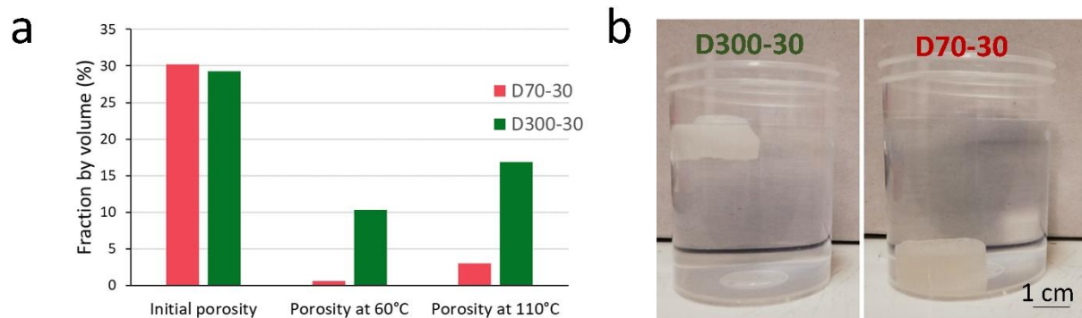
Figure 6 – a) Characteristics of the dried thick samples with different pore sizes; b) a photograph of the dried samples demonstrating flotation (D300-30) and sinking (D70-30) in pure water.
