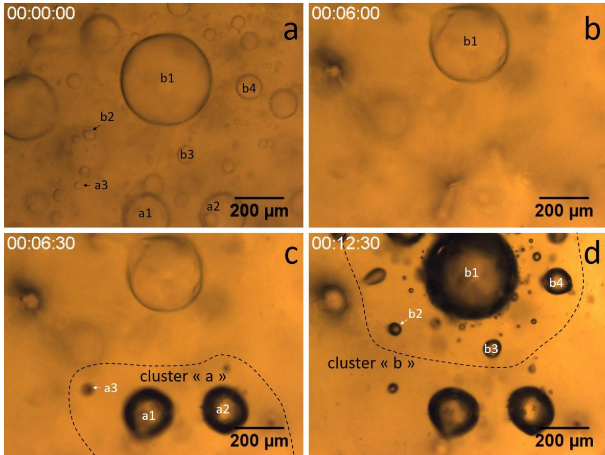
Figure 8 – Optical microscopy images of different drying stages of porous PDMS sample with 5% porosity at 110°C. Symbols a1-a3 and b1-b4 mark similar pores in zones a and b, respectively, before and after cavitation.
