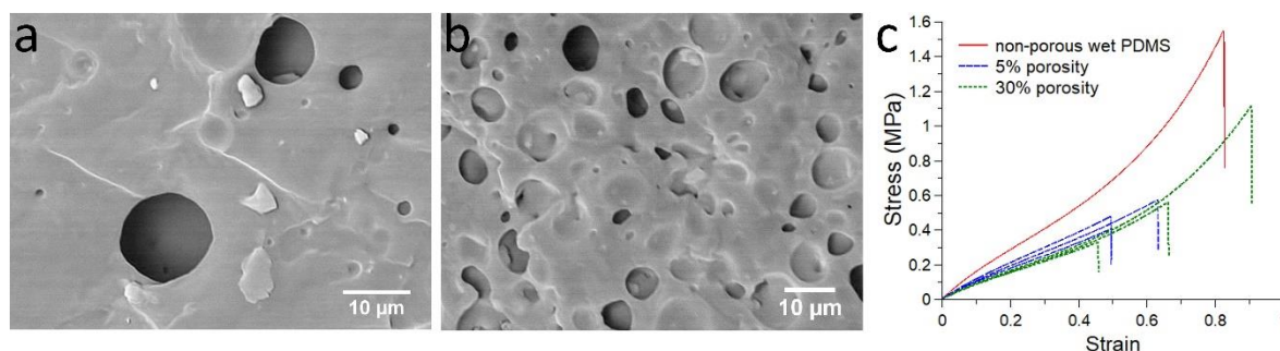
Figure 1 – a) and b) Scanning electron microscopy images of sections of the sample D200-5 with 5% porosity (a) and sample D70-30 with 30% porosity (b). c) Stress-strain curves of the same samples in wet state in comparison with a non-porous PDMS “swollen” in water at 60°C for 6 hours (red curve). For each type of porous sample, the measurement was performed on 3 samples.
