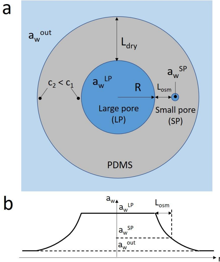
Figure 11 –a) The model used to estimate the osmotic length L_{osm} : a small spherical pore “SP” with high concentration of NaCl is located near a large spherical pore “LP” in a PDMS shell of thickness L_{dry} . a_w^{LP} and a_w^{SP} and a_w^{out} are the activities of water in the large pore, small pore and outside medium, respectively; c_1 and c_2 design the water concentrations in PDMS near the large pore and near the border. The schematic is not drawn to scale, in the sense that the characteristic distance L_{dry} of the large pore to the edge of the sample is, for most pores, much larger than the size of the pore b) The corresponding schematic of the radial distribution of water activity in the shell, when neglecting the impact of the small pore “SP”.
