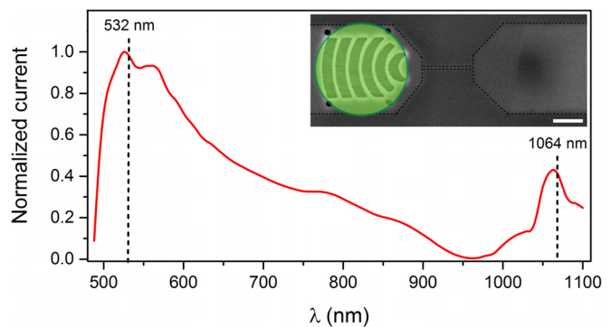
FIG. 2. Spectral responsivity of the FGC excited by a tunable laser, operating in the wavelength range between \lambda = 480 nm and 1100 nm, while simultaneously biasing the device with V_{\text{Bias}} = 100 mV. The diameter and length of the c-Al NW waveguide attached to the FGC were 40 nm and 700 nm, respectively. The measurement was conducted at room temperature and ambient conditions, and the data were corrected with respect to the wavelength dependent laser output power. The SEM image in the inset shows the overall contact arrangement of the Al-Ge-Al NW heterostructure device. The scale bar is 1 \mu\text{m} . The green spot indicates the laser position for exciting the FGC by the tunable laser.
