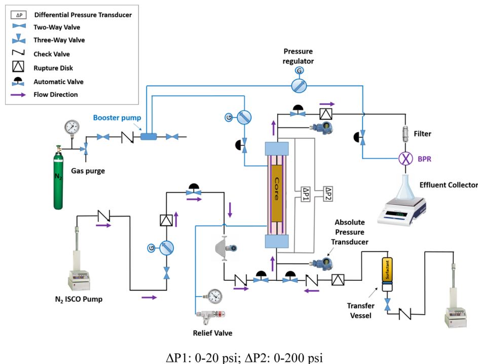
Figure 1. Schematic diagram of the Grace M9300 core flooding apparatus for proposed nitrogen/surfactant solution coinjection process.
