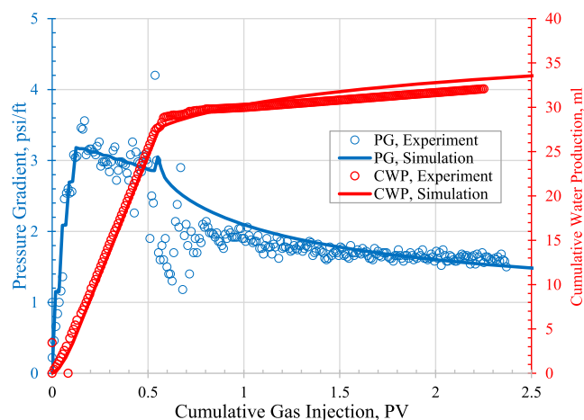
Figure 3. PG and cumulative water production during the CGI process at 4 ft/d for both simulations (solid lines) and experimental measurements (points).
