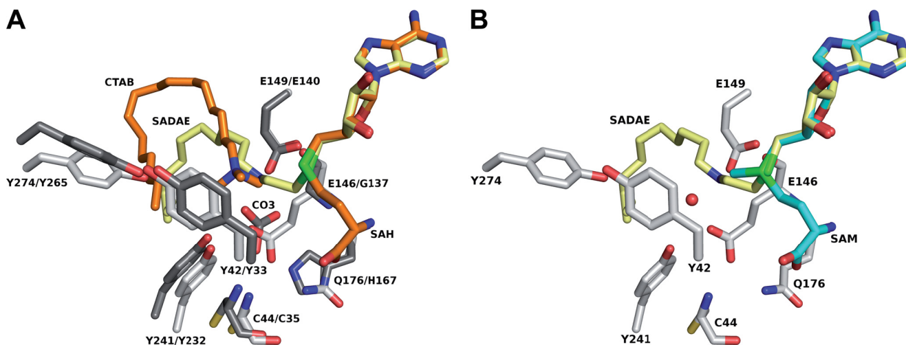
FIGURE 8. Active-site architecture of MA-MTs. A, chemical environment of SADAE in Hma and of AdoHcy and a cationic lipid, as observed in the structure of MmaA2-AdoHcy-CTAB (Protein Data Bank code 1TPY). B, superimposition of SADAE and AdoMet from the Hma-AdoMet complex (Protein Data Bank code 2FK8). Color code is as follows: Hma, light gray carbon atoms; MmaA2, dark gray carbon atoms; SADAE, yellow carbon atoms; AdoHcy and CTAB, orange carbon atoms; AdoMet, cyan carbon atoms. The Hma-AdoMet active site water molecule discussed in the text is represented as a red sphere. Residue numbering: Hma/MmaA2.
