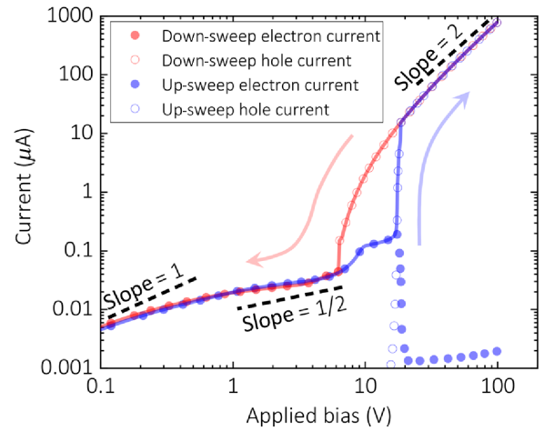
FIG. 6. The calculated current-voltage characteristics (solid lines) calculated using a self-consistent solution of the Poisson-transport equations [40]. The colors correspond to the voltage sweep direction as indicated by the arrows, and the symbols illustrate the switch from an electron to a hole current at V_t . The model qualitatively reproduces the punch-through behavior observed experimentally in Fig. 4.
