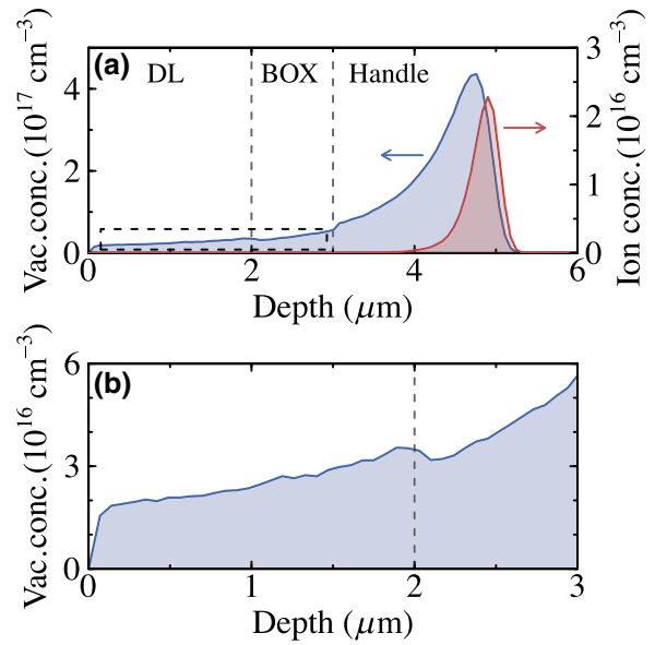
FIG. 2. (a) SRIM modeling of the 10 MeV \text{Si}^{5+} ion implant into the silicon-on-insulator wafers. The implant principally occurs in the wafer handle (red curve in the top panel), but a long tail of implanted ions on the device layer side results in an approximately homogeneous distribution of silicon divacancy defects of density approximately 2.5 \times 10^{16} \text{ cm}^{-3} in the device layer itself [blue curves, including the enlarged device layer view in (b)].
