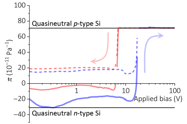
FIG. 8. PZR calculated using the self-consistent Poisson and drift-diffusion equation solver for the up- and down-voltage sweeps as indicated by the colors and arrows. A stress-induced change in the effective masses alone [19] does not result in anomalous PZR at low bias (dashed lines), but stress-induced shifts in the trap energies consistent with known band deformation potentials do however (solid lines). The curves show many qualitative similarities with the measured data in Fig. 7(a).
