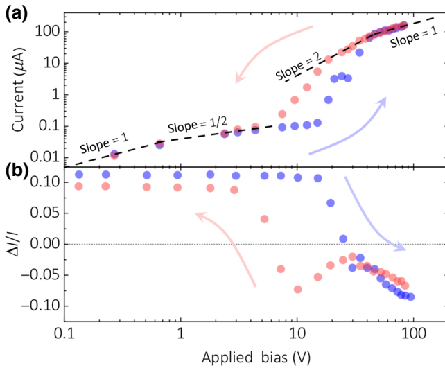
FIG. 4. (a) Experimentally measured up- (blue circles and arrow) and down- (red circles and arrow) sweep current-voltage characteristics obtained on the defect engineered devices. The slopes indicated in the log-log plot are a guide to the eye. (b) Relative current change induced by a +1 V change in the voltage applied to the wafer handle. The sign indicates a majority electron current below a threshold voltage, V_t , and a majority hole current above this bias. A hysteresis in V_t is clearly visible between the up and down sweeps.
