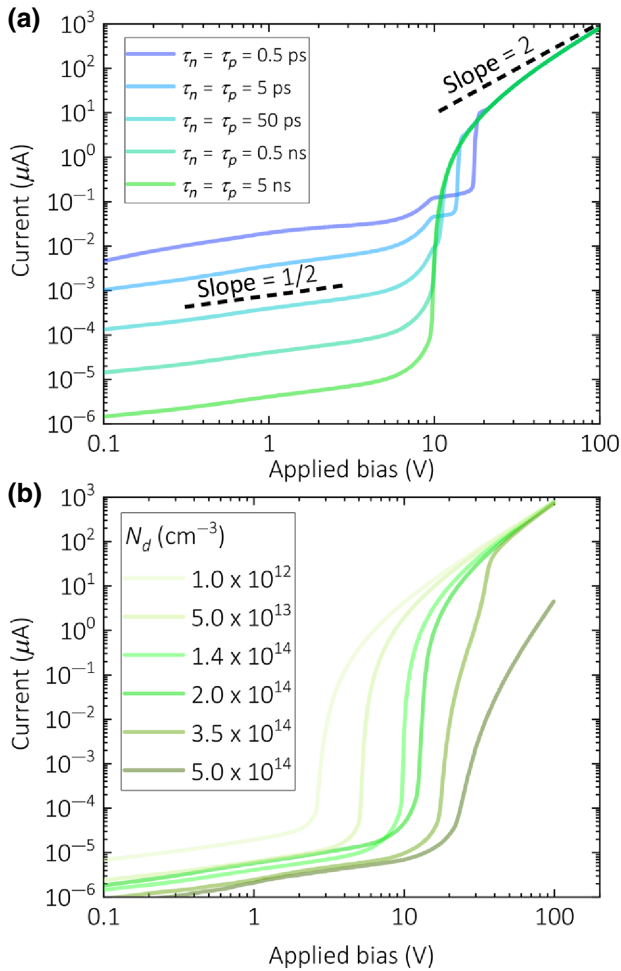
FIG. 5. Calculated dependence of the device characteristics on (a) the SRH recombination times \tau_n and \tau_p for a donor density N_d = 1.4 \times 10^{14} \text{ cm}^{-3} and (b) the donor density N_d for \tau_n = \tau_p = 5 \text{ ns} . The lifetimes principally change the subthreshold electron current that is recombination limited, and N_d principally changes the threshold voltage V_t corresponding to the rapid increase in current and the onset of a space-charge-limited hole current.
