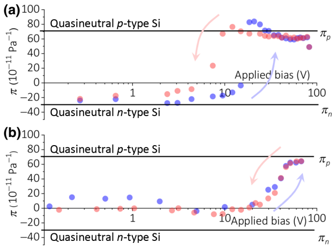
FIG. 7. PZR \pi coefficient measured under 20 MPa of uniaxial tensile stress parallel to the applied current along the \langle 110 \rangle crystal direction. Up (blue circles and arrow) and down (red circles and arrow) sweeps are shown. (a) Results from the defect-engineered sample whose characteristics are shown in Fig. 4. Near V_t , \pi changes sign and is approximately bounded by the known bulk silicon values [19] given in Eqs. (2) and (3). (b) Results for a device prior to defect engineering. No anomalous (negative) PZR is observed. Note also that the hysteresis is only present in defect-engineered devices.
