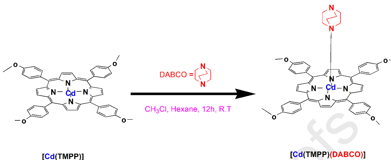
Scheme 2: Synthetic route to [Cd(TMPP)(DABCO)] complex ( I ).
