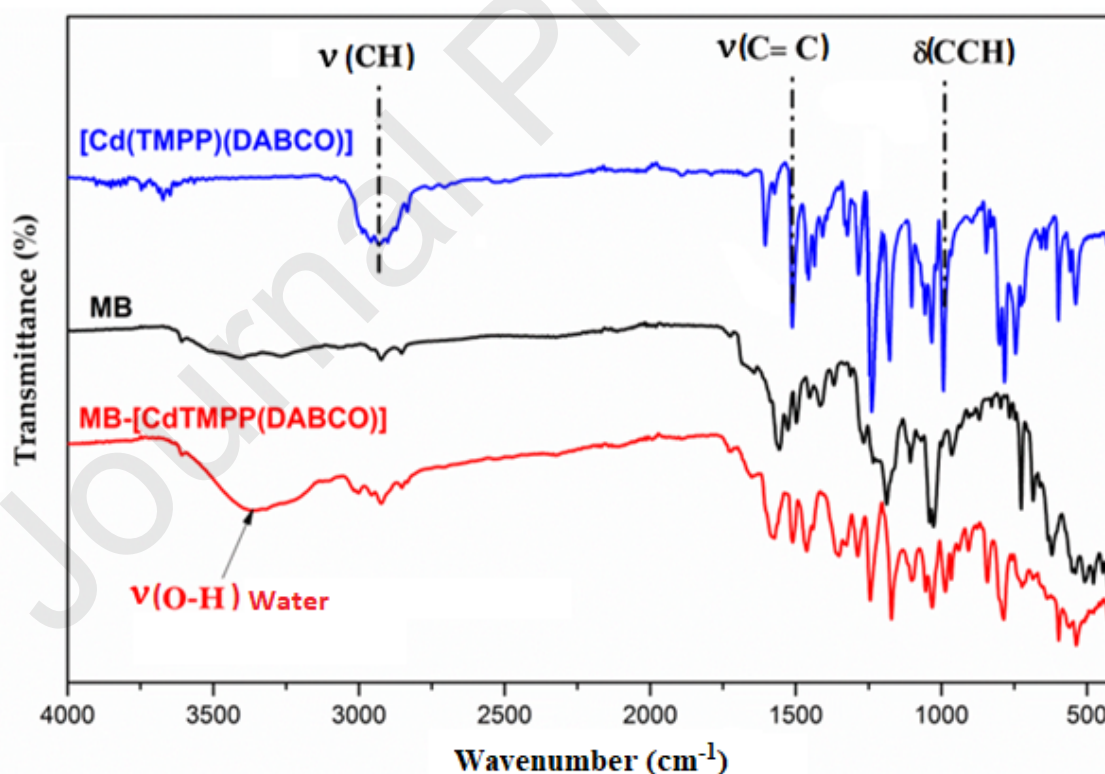
Figure 8. FT-IR spectra of [ Cd(TMPP)(DABCO)], MB, and MB-[Cd(TMPP)(DABCO)].
