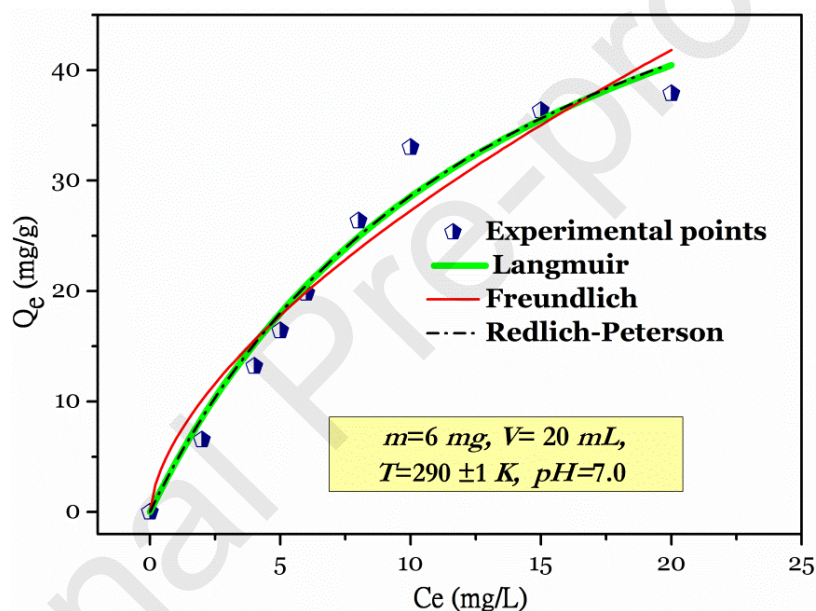
Figure 7. Adsorption isotherms of MB dye onto [Cd(TMPP)(DABCO)] (I) and fitting curves of the selective models.
