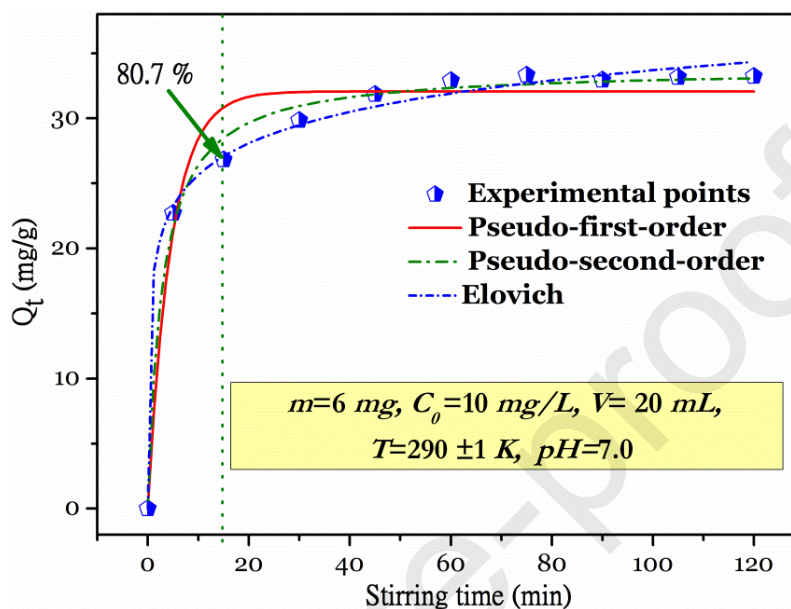
Figure 6. MB dye ( C_0 = 10 \text{ mg.L}^{-1} ) as a function of time for complex (I) ( m = 6 \text{ mg} , \text{pH} = 7.0 ). Dots represents the experimental data and the curves where plotted using the pseudo-first-order, the pseudo-second-order and the Elovich models.
