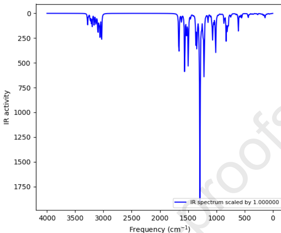
Figure 4. Theoretical IR spectra of the complex (I).
