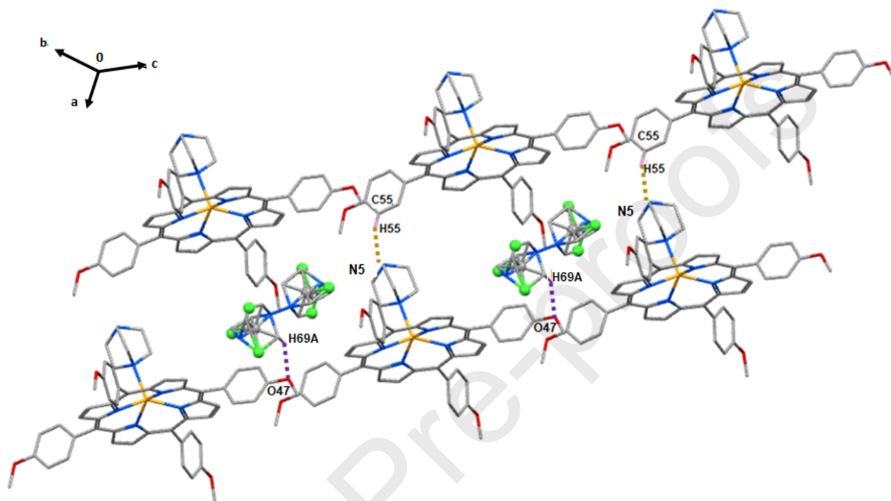
Figure 3. Schematic representation of the pseudo-2D supramolecular architecture of complex (I) via C–H⋯N and C–H⋯O interactions. Only relevant atoms have been shown.
