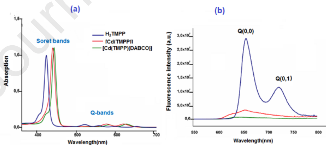
Figure 5. (a) UV-Visible spectra of H_2TMPP , [Cd(TMPP)] and complex (I) in CH_2Cl_2 ( c \sim 10^{-5} M), (b) fluorescence emission spectra of the same three porphyrinic species in CH_2Cl_2 ( c \sim 10^{-6} M), excitation \lambda_{exc} = 437 nm.
