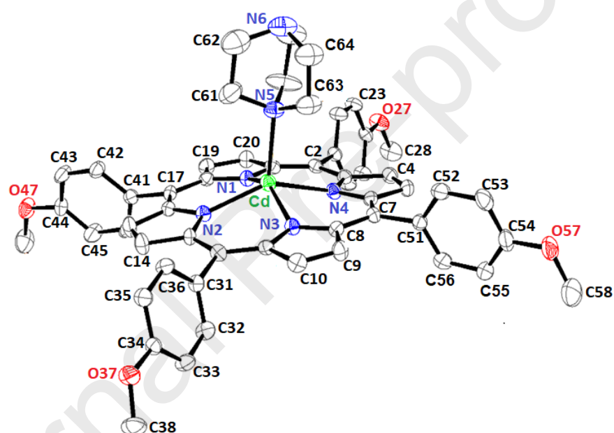
Figure 1. ORTEP diagram and numbering scheme of [Cd(TMPP)(DABCO)] . The hydrogen atoms are not represented for clarity. 30% probability surfaces.
