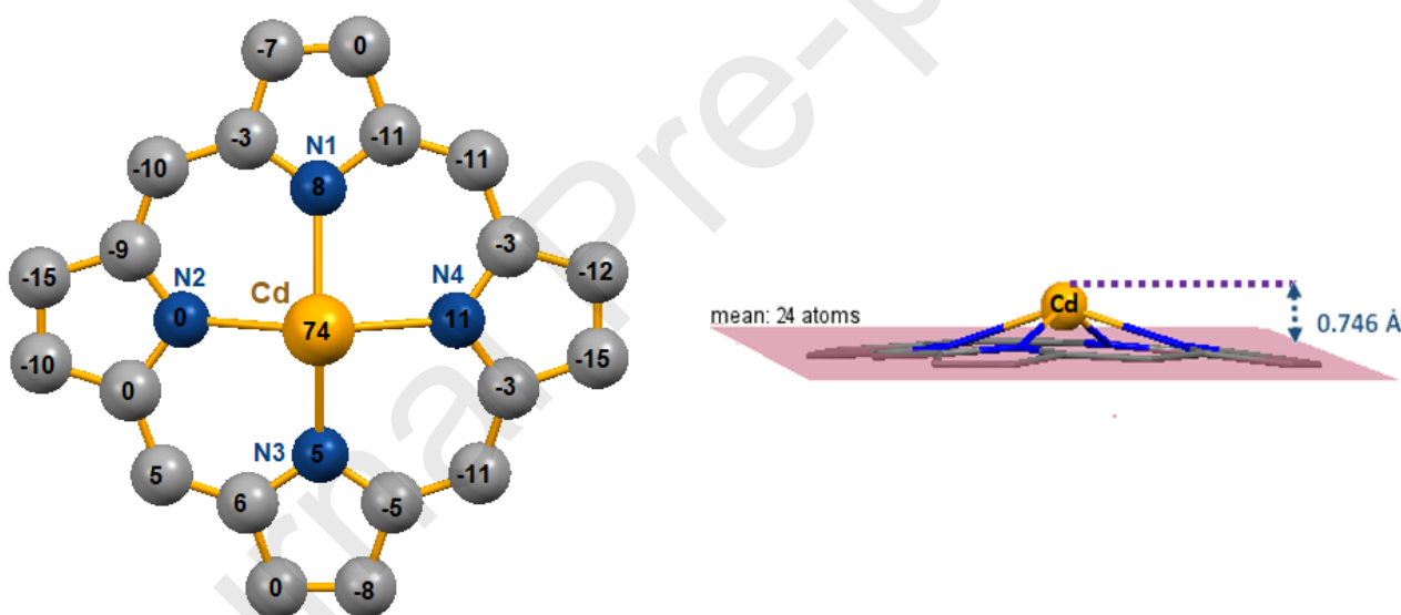
Figure 2. Formal diagrams of the porphyrinato core showing the Doming distortion in [Cd(TMPP)DABCO] complex ( I )
