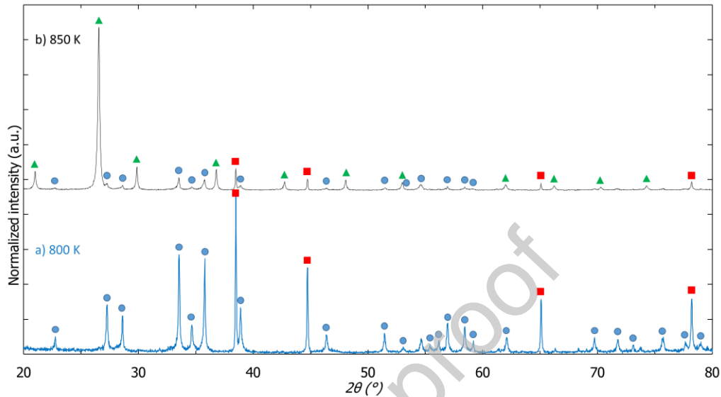
Fig. 3 X-ray diffraction patterns acquired on the surface of an \text{U}_3\text{Si}_2+\text{Al} fuel meat sintered at 76 MPa, with a dwell time of 5 minutes and an uranium loading of 5.6 \text{ g}_\text{U} \text{ cm}^{-3} at (a) 800 K and (b) 850 K. The diffraction peaks are indexed with \bullet \text{U}_3\text{Si}_2 , \blacksquare Al and \blacktriangle \text{U}(\text{Al},\text{Si})_3 diffraction peaks.
