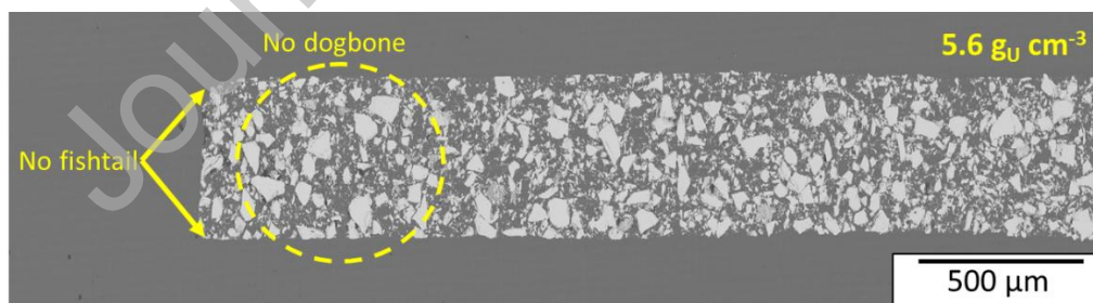
SEM image of a cross section of a nuclear fuel plate edge manufactured by SPS
