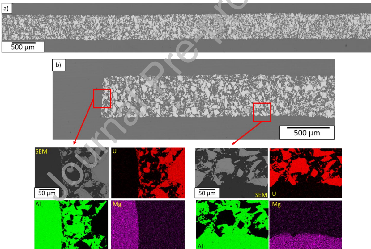
Fig. 5 (a) Stacked backscattered electron SEM images of a cross section of a U_3Si_2 -based fuel plate manufactured by SPS, (b) Backscattered electron SEM images of the extremity of the plate and EDS X-ray maps acquired in areas boxed in red
