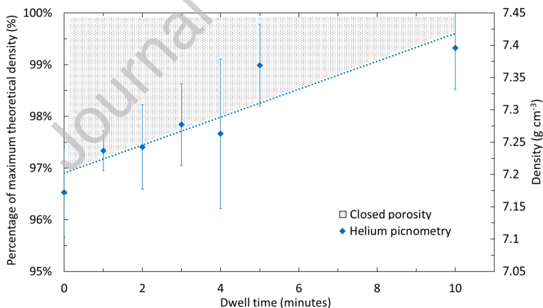
Fig. 4 He-pycnometry density (right axis) and its equivalent percentage of the maximum theoretical density ( 7.45 \text{ g cm}^{-3} for a uranium loading of 5.6 \text{ g}_U \text{ cm}^{-3} , left axis) of \text{U}_3\text{Si}_2 +Al fuel meats prepared by SPS, as a function of dwell time at 800 K - 76 MPa
