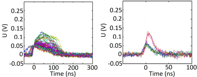
Fig. 7. Representatives pulses obtained with a fission chamber taken from [17]. Left: ^{252}\text{Cf} neutron-induced pulses at room temperature. Right: PD-induced pulses at 600 °C.
