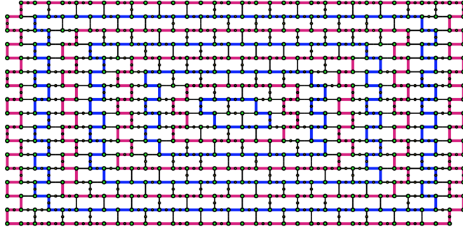
Figure 1: A 17-wall and its 8 layers.
