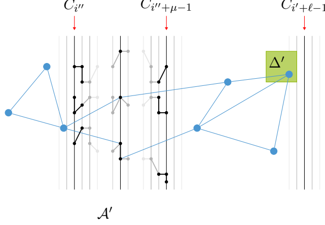
Figure 8: An example of (\tilde{M}, \tilde{T}) , the result of applying Theorem 3 in the railed annulus \mathcal{A}' .
