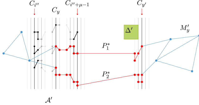
Figure 10: Visualization of the last part of the proof.
