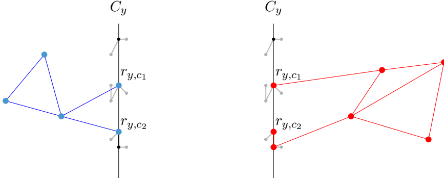
Figure 9: The graphs M_y (depicted in red) and \hat{M}_y (depicted in blue).
