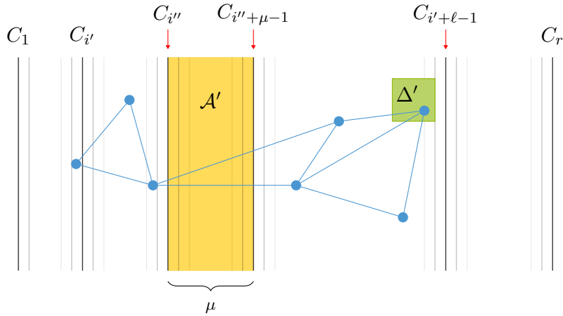
Figure 7: An example showing the (\mu, q) -railed annulus \mathcal{A}' .
