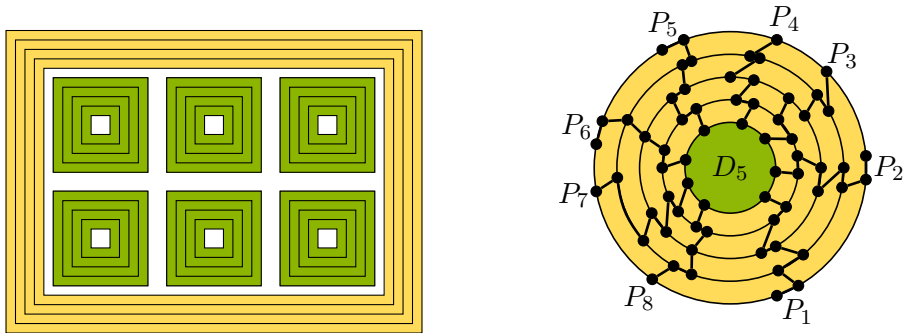
Figure 2: Left: The partition of a wall into a yellow annulus and several green subwalls. Right: An example of a (5, 8) -railed annulus depicted in yellow; its inner disk D_5 is depicted in green.
