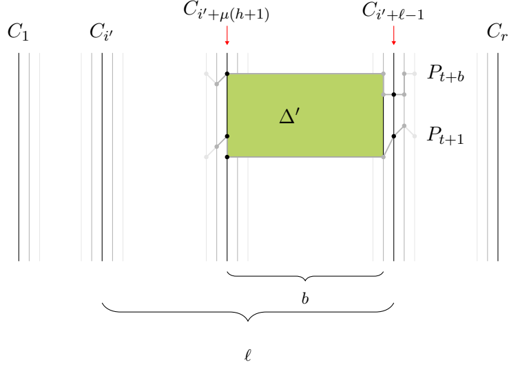
Figure 6: An example showing the disk \Delta' .
