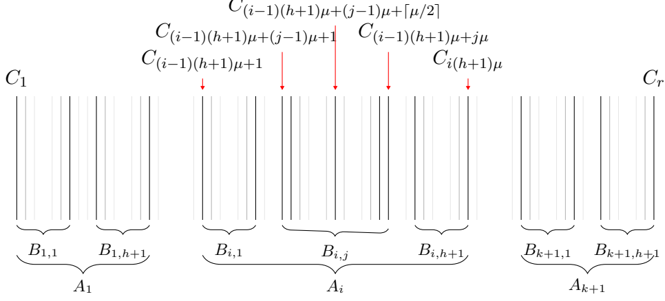
Figure 3: Visualization of the partition of the cycles of \mathcal{A} in sets A_i, i \in [k+1] and of the partition in sets B_{i,j}, i, j \in [k+1] \times [h+1] .
