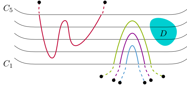
Figure 13: An example of a (\mathcal{C}, D, L) -valley (depicted in solid red), and some (\mathcal{C}, D, L) -mountains (depicted in solid colors). Notice that the (\mathcal{C}, D, L) -mountain depicted in green is tight.
