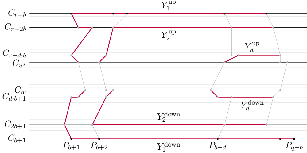
Figure 21: Visualization of the definition of Y_i^{\text{up}} and Y_i^{\text{down}} , i \in [d] .
