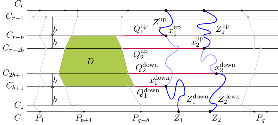
Figure 20: Visualization of an (r, q) -railed annulus and the notations introduced above.
