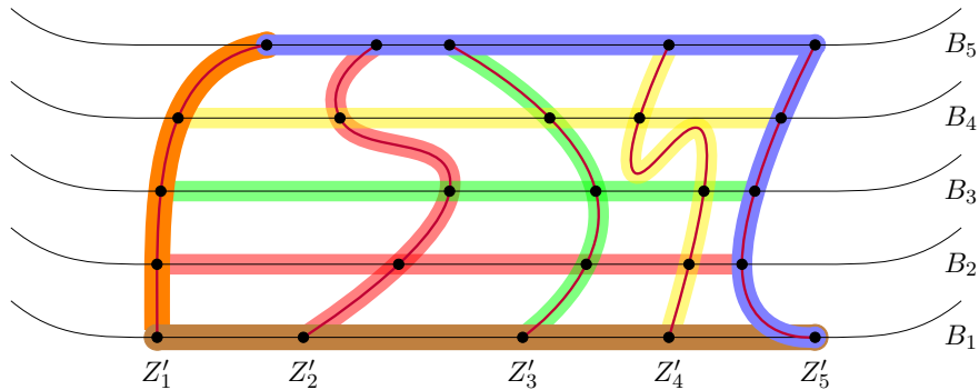
Figure 16: An example of the construction of a bramble of Q , where |\mathcal{B}| = 5 and |\mathcal{Z}'| = 5 . Here, X^{(2,2)}, X^{(3,3)}, X^{(4,4)} are depicted in red, green, and yellow, respectively, while X^{(1)}, X^{(2)}, X^{(3)} are depicted in orange, brown, and blue, respectively.
