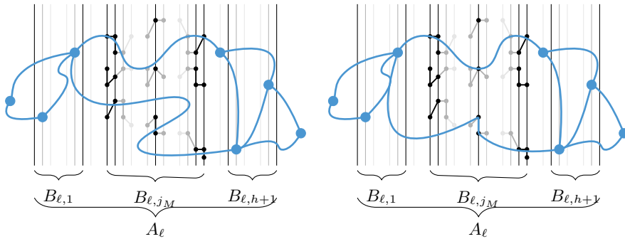
Figure 4: Visualization of the statement of the Claim. (M, T) is depicted in the left figure, while (\tilde{M}, \tilde{T}) is depicted in the right figure.
