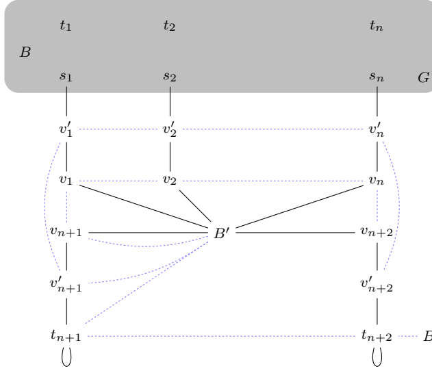
Fig. 4: Reduction of \mathbf{Reachability-init}_{\text{und}} into \mathbf{Reachability}_{\text{und}} . The node t_{n+2} communicates with all nodes v such that v communicates with B .
