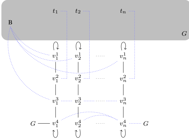
Fig. 5: Reduction of \mathbf{Reachability}_{\text{und}} to \mathbf{Coverage-init}_{\text{und}} .
