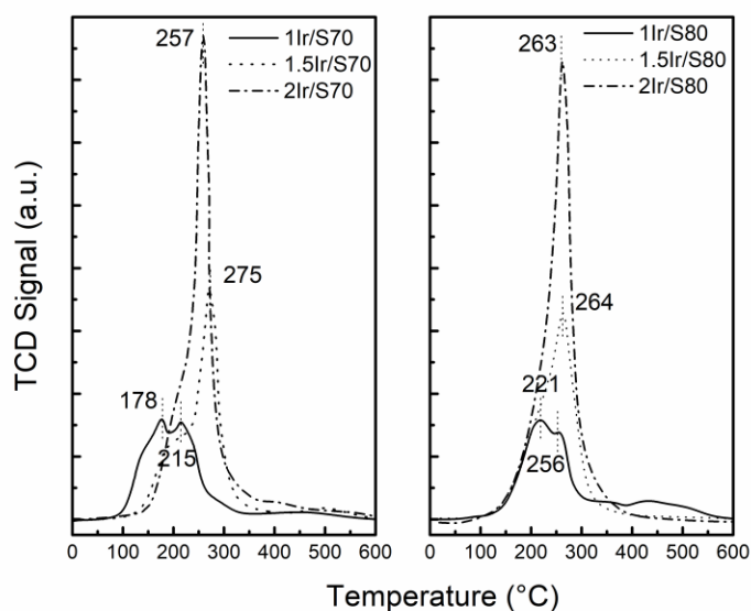
Figure 3. TPR traces of both catalyst series.
