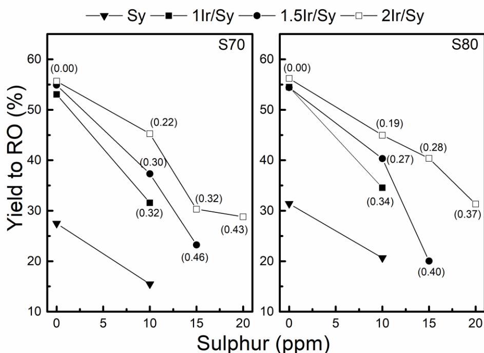
Figure 9. Yield to ring opening products as a function of the S content on decalin reaction obtained at 6 h reaction ( T = 350\text{ }^{\circ}\text{C} ). Values between brackets correspond to the S/Ir_{\text{surf}} ratio.
