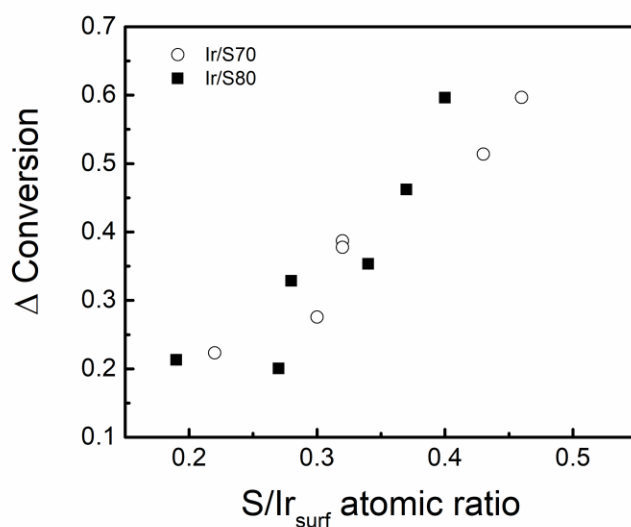
Figure 7. Relative conversion loss due to sulphur as a function of S/Ir surf for both catalysts series. ( \Delta\text{conversion} = (X_{\text{pure decalin}} - X_{\text{decalin with S}})/X_{\text{pure decalin}} ).
