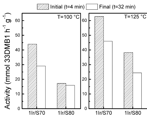
Figure 2. Initial and final activity on the isomerization of 33DMB1 reaction at reaction temperature 100 and 125 °C.
