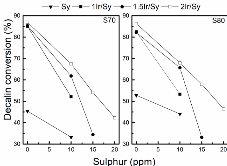
Figure 6. Conversion as a function of the sulphur content (ppm) obtained on decalin reaction at 350 °C.
