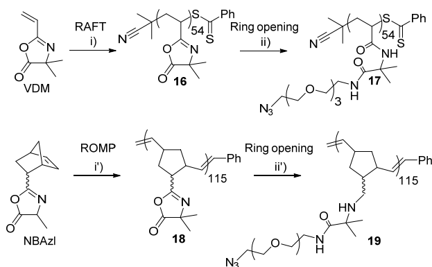
Scheme 2. Synthesis of azido-polymers 17 and 19 from VDM and NBAzl. i) 2-cyanoprop-2-ylbenzodithioate, AIBN 60°C, 24h, 35% ii) 11-Azido-3,6,9-trioxaundecan-1-amine, THF, 40°C, 26h, quant.
