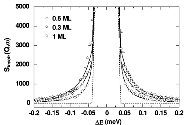
FIG. 5. Evolution of the QENS spectra at Q = 1.110 \text{ Å}^{-1} vs HCl coverage. Experimental spectra are represented by empty symbols and the solid lines are the best fits for each HCl coverage. The dashed line represents the experimental resolution.
