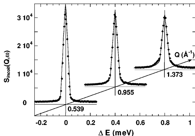
FIG. 4. Evolution of the QENS spectra measured at T = 250 K vs the scattering vector, for an HCl coverage \Theta_{\text{HCl}} = 0.6 ML. Experimental spectra are represented by full diamond symbols and the solid lines are the best fits.
