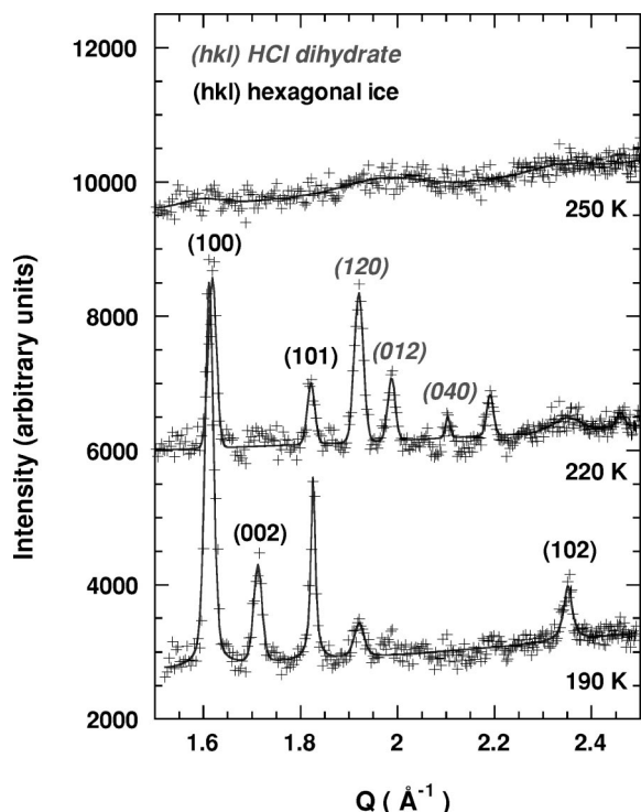
FIG. 3. Evolution of the neutron diffractograms of the 5 BL ice film with an HCl coverage of \Theta_{\text{HCl}} = 1 ML vs temperature. Experimental spectra are represented by crosses and the solid lines are the best fits. Peak (hkl) written in italic correspond to the dihydrate phase.
