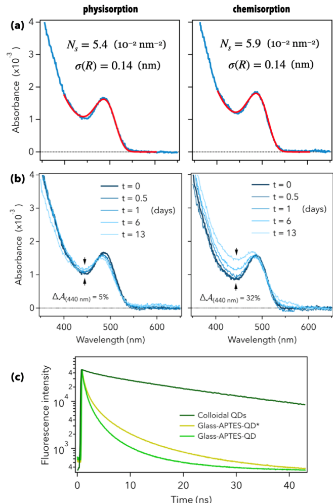
Figure 4. (a) UV-visible spectra of Glass-APTES-QD samples obtained without activation of QDs (left column) and of Glass-APTES-QD* samples obtained with activation of QDs by EDC-NHS (right column). The red curves are fits to the experimental data (see Supporting Information, section II). Here, the surface density N_s of QDs and their radius dispersion \sigma(R) are the fitting parameters. (b) Kinetic study of the UV-visible extinction spectra of non-activated (left) and activated (right) samples. The time t = 0 corresponds to the time after the samples are taken out of their QD baths, rinsed and dried. For each sample, we calculate \Delta A_{487\text{nm}} as explained in the text and detailed in Supporting Information (section II, Fig. C). (c) Time-resolved measurements of the fluorescence emitted by CdTe QDs in colloidal solution and in monolayers, both on Glass-APTES-QD and Glass-APTES-QD* samples (for t = 0 ).
