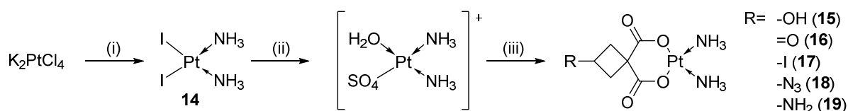
Scheme 2: Reagents and conditions: (i) KI, H 2 O, then NH 4 OH, r.t., 89%; (ii) Ag 2 SO 4 , H 2 O, dark, r.t., not isolated; (iii) Ba(OH) 2 , 9-13 , r.t., 79% (15), 52% (16), 39% (17), 31% (18); 3% (19).
