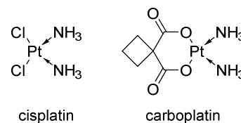
Figure 1: Structures of cisplatin and carboplatin
