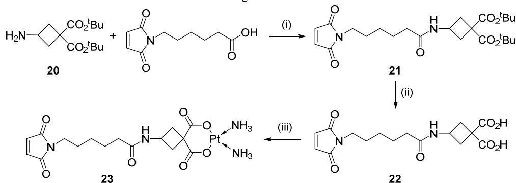
Scheme 3: Reagents and conditions: (i) HATU, 2,6-lutidine, DMF, r.t., 89%; (ii) TFA, DCM, r.t., 92%; (iii) Pt(NH_3)_2I_2 , AgSO_4 , H_2O , then Ba(OH)_2 , 23 , r.t., 30%
