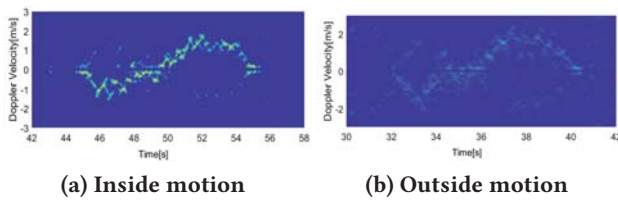
Figure 4: Doppler velocity spectrum when human motion occurs inside and outside the house
