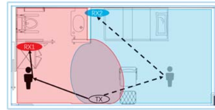
Figure 5: Sensing area of different Wi-Fi devices Table 1: Intrusion results combined from two devices
