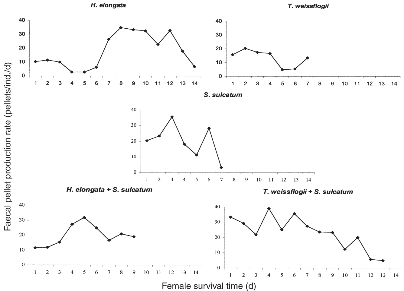
Fig. 6. Centropages typicus . Faecal pellet production rate as a function of female survival time (d) for the different diets
