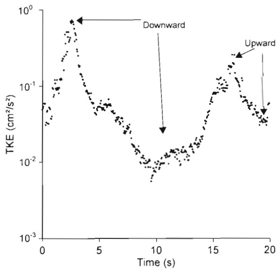
Fig. 1. Time series measurement of turbulent kinetic energy, TKE ( \text{cm}^2 \text{s}^{-2} ), over a period of oscillation of the grid at 3 strokes \text{min}^{-1} . The 2 peaks of kinetic energy indicate the downward and upward passages of the grid during the oscillation period. Arrows indicate fractions of the oscillation period showing a decrease of TKE over time which are used to compute \langle \epsilon \rangle (see text and Table 1 for further details)
