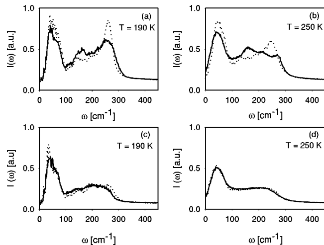
FIG. 7. Power spectrum (in arbitrary unit) of the linear velocity autocorrelation function for the water molecules at two temperatures: (a) and (b) for the whole film, and (c) and (d) for the outermost bilayer. Full curves correspond to the supported film phonon density of states and dotted curves to bulk ice phonons.
