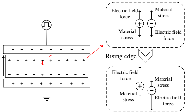
(b) Change in the forces at the rising edge (from -15 to -30 kV/mm).
