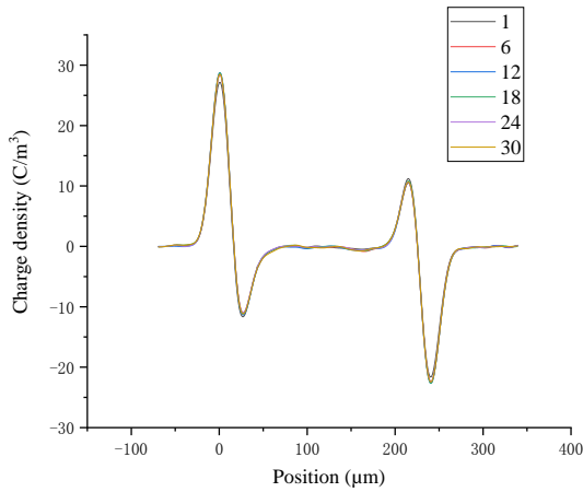
Fig. 10. Change in space charge at a low-voltage level of -15 kV/mm applied for 2 h.
