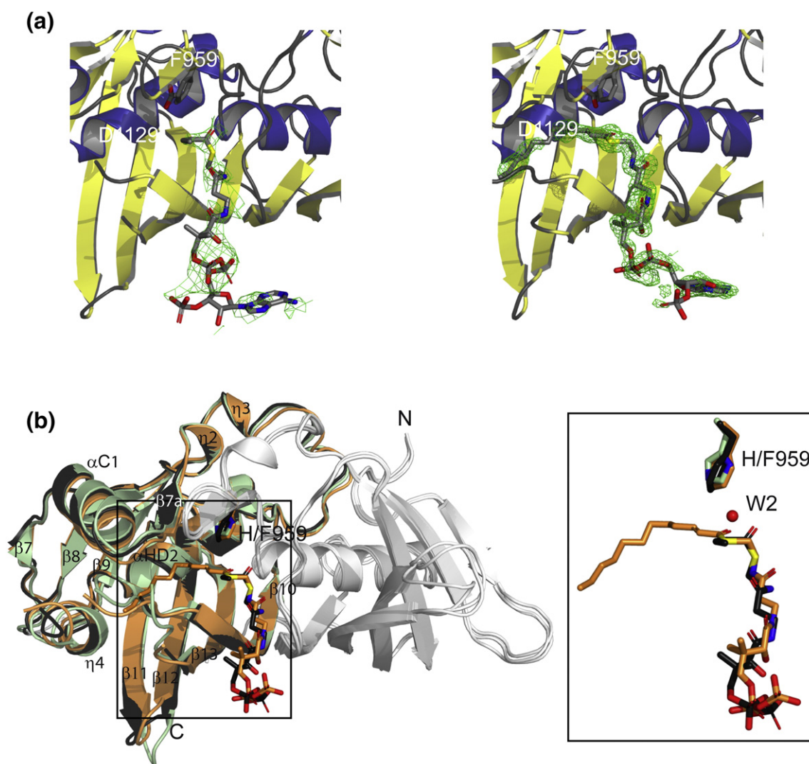
Fig. 5. Structural alignment of the DH_{PpsC} structures. (a) The active site histidine (H959) has been mutated into a phenylalanine (F959). Simulated-annealing 2Fo-Fc composite omit electron density maps contoured at 1.0\sigma around the CoA derivatives are shown in green for DH_{PpsC} in complex with C_{4:1} -CoA (left) and C_{12:1} -CoA (right). For clarity, only one alternate conformation is shown for the 3',5'-ADP moiety of C_{12:1} -CoA outside the cavity. (b) The C-terminal hot dog domain of wild-type apo- DH_{PpsC} (green) is superimposed onto the DH_{PpsC}/C_{4:1} -CoA (black) and DH_{PpsC}/C_{12:1} -CoA (orange) structures. The same color code is used for the carbon atoms of CoA derivatives and the active site residues H959 and F959. The N-terminal hotdog is in white for all three structures. Secondary structure elements delineating the tunnel cavity are indicated. Closeup view of the superimposition between the C_{4:1} -CoA (black) and C_{12:1} -CoA (orange).
