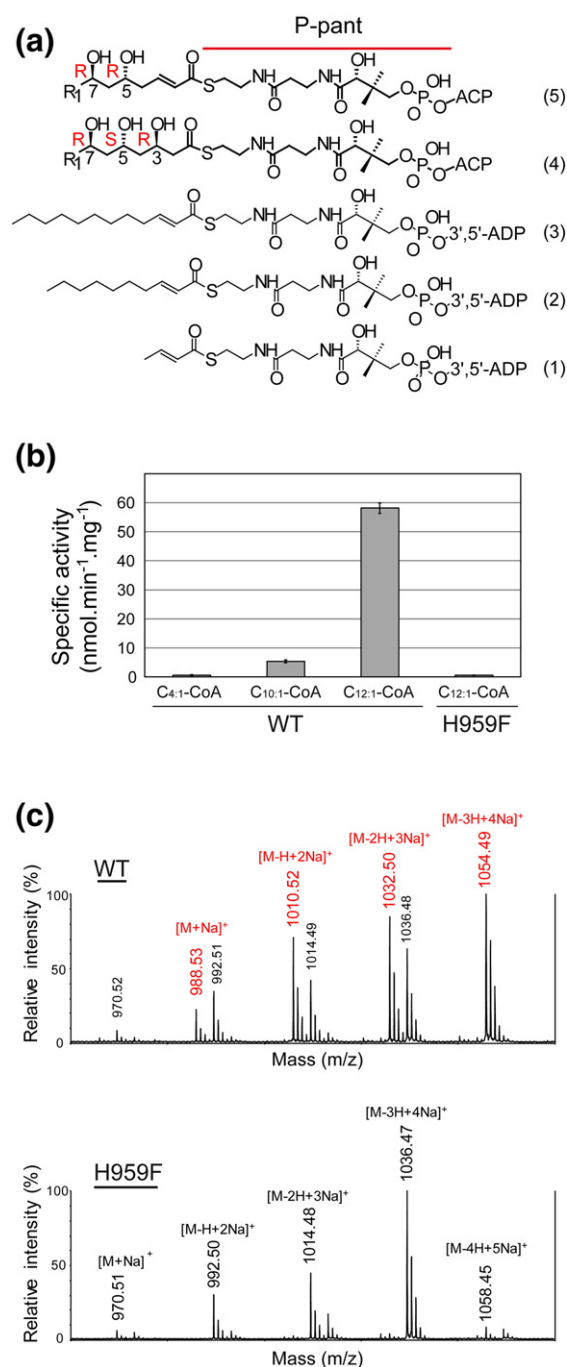
Fig. 4. Activity assays. Enzyme assays were performed on the wild-type DH PpsC and H959F mutant using (1) trans -but-2-enoyl-CoA (C 4:1 -CoA), (2) trans -dec-2-enoyl-CoA (C 10:1 -CoA), and (3) trans -dodec-2-enoyl-CoA (C 12:1 -CoA). The natural substrate (5) and dehydration product (4) are also depicted. R 1 = CH 3 -(CH 2 ) 20-22 . (b) Disappearance of the C=C double bond at 263 nm was detected in the presence of C 10:1 -CoA and C 12:1 -CoA. (c) The hydrated product was confirmed from MALDI-TOF MS experiments with the wild-type enzyme (top). No product was detected for the H959F variant (bottom). The substrate ion peaks are labeled in black and the hydration product ion peaks are labeled in red.
