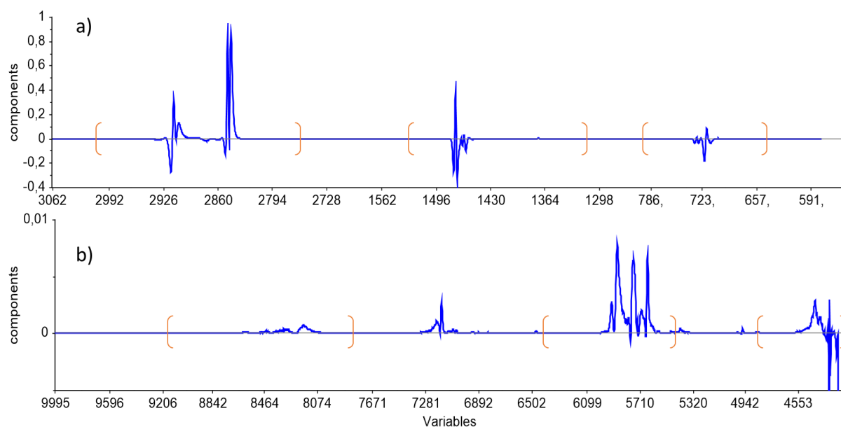
Figure 6. The contribution plot describes how individual variables contribute to the model, 3 spectral regions were clearly highlighted a) in MIR and b) in NIR. Variables represents the wavelength in \text{cm}^{-1} . The brackets indicate the wavelength ranges selected to be included in the models.
