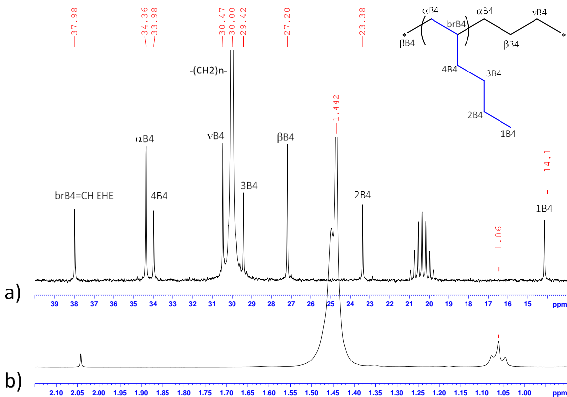
Figure 1. ^{13}\text{C} NMR spectra (TCB/ toluene- d_8 , 363 K) of sample 23 with 2,2 mol% of 1-hexene, a), resonance region of ^1\text{H} NMR spectra (TCB/ toluene- d_8 , 363 K) of sample 40 with 13,6 mol% of 1-hexene b).
