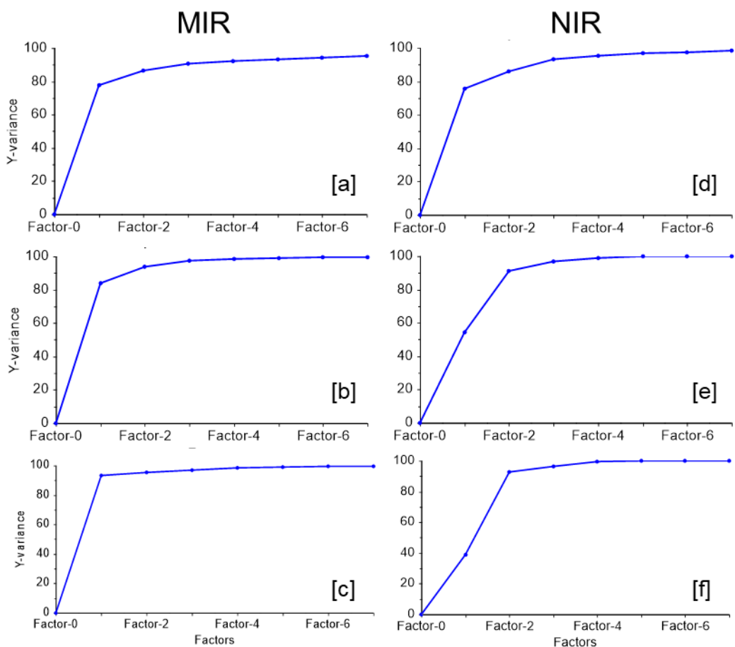
Figure 7. Evolution of performance index (in %) in function of the number of PLS factors for the six models reported in Table 3.
