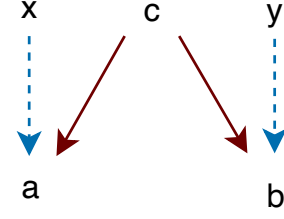
Figure 2: Graph \mathbf{G} from Example 1.
