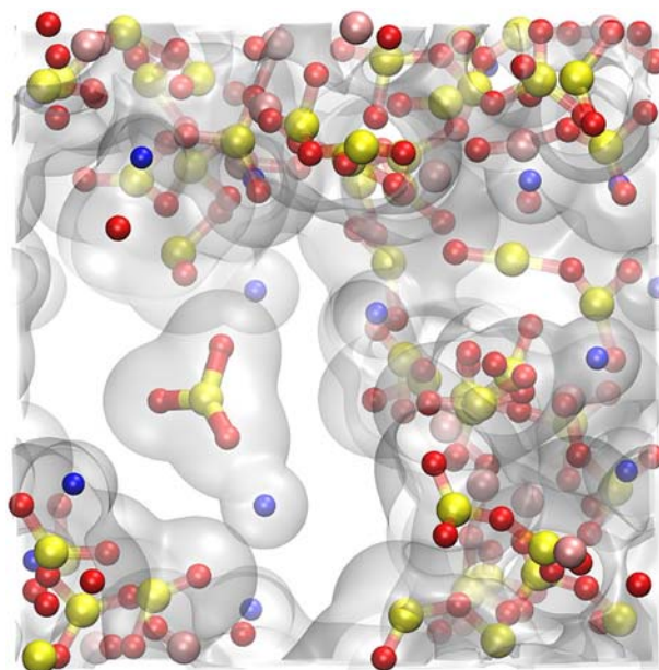
Figure 8. Snapshot of the iso-electronic density surface at 0.01 \text{ e}/\text{\AA}^3 in the simulation cell at 4000 K and 1.02 \text{ g cm}^{-3} created with VMD (Humphrey et al., 1996). We see a clear bubble with a \text{NaSiO}_3 cluster inside. Colors indicate elements: red = O, yellow = Si, pink = Al, and blue = Na.
