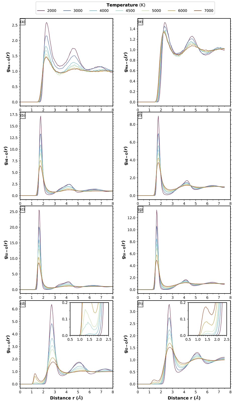
Figure 3. Pair distribution function of X-O (X being Na, Al, Si, and O) in \text{NaAlSi}_3\text{O}_8 at 1.02 \text{ g cm}^{-3} (a-d) and 2.06 \text{ g cm}^{-3} (e-h). Colors indicate temperatures. The insert shows a zoom on the region 0.5\text{--}2.5 \text{ \AA} . The small peak located around 1.4 \text{ \AA} marks the presence of \text{O}_2 molecules.
