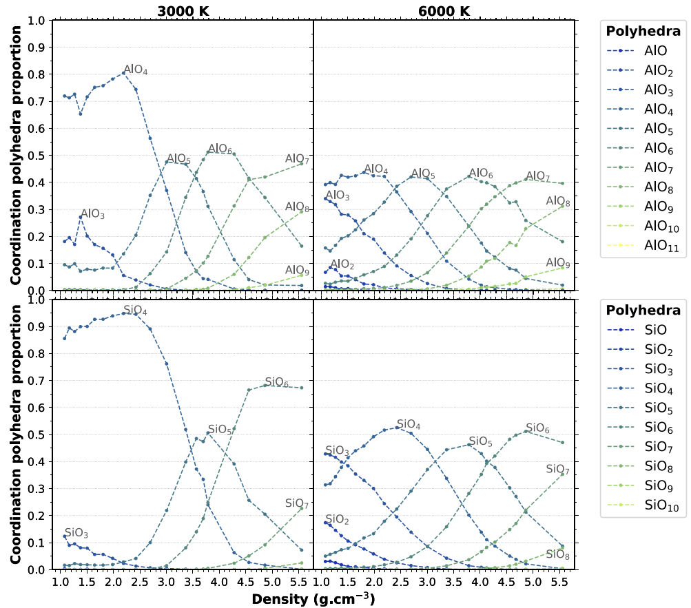
Figure 6. Relative proportion of \text{SiO}_x and \text{AlO}_x coordination species in \text{KAlSi}_3\text{O}_8 for 3000 and 6000 K as a function of density.
