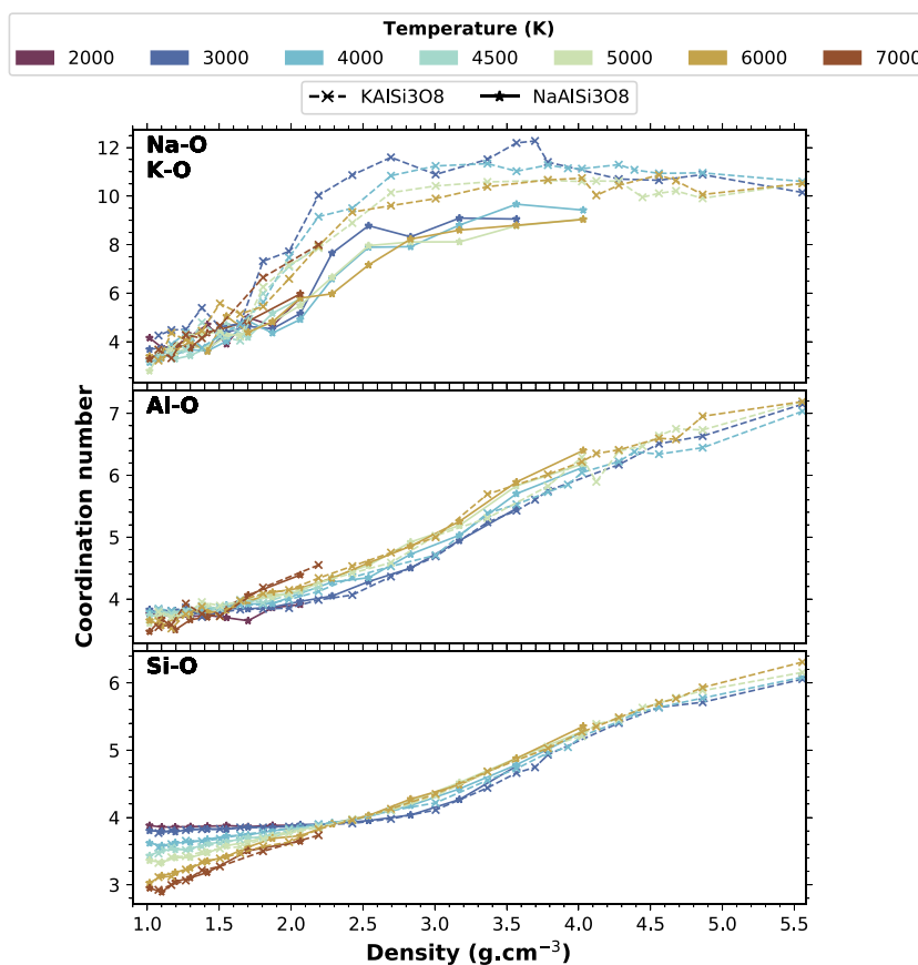
Figure 4. Average coordination number of Na, K, Al, and Si by O for the Na-feldspar (stars and continuous lines) and K-feldspar (crosses and dashed lines). At ambient conditions the solid or glass feldspars have \text{NaO}_{6-9} , \text{KO}_9 , \text{AlO}_4 , and \text{SiO}_4 coordination polyhedra (Jackson et al., 1987; Muller et al., 1993; Ribbe, 1984; Xue & Stebbins, 1993). Colors indicate temperature.
