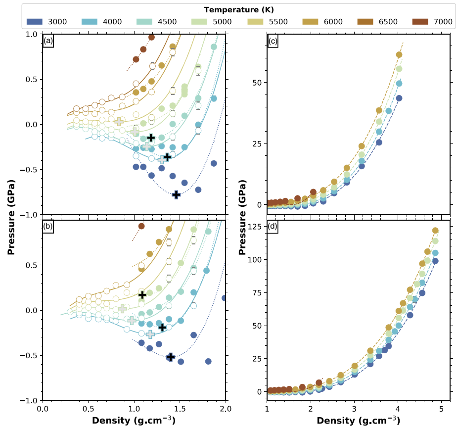
Figure 2. Computed pressure as a function of density around the spinodal part of the phase diagram for the (a) Na-feldspar and (b) K-feldspar end-members and their respective view on the complete density range studied here, (c) and (d). Colors indicate temperature. Open symbols indicate values obtained with pseudopotentials which require a lower plane wave energy cutoff than those used to obtain the data set of solid symbols. Solid and dotted lines represent the third-order polynomial curve fits corresponding to the respective two sets of data. The open and solid crosses indicate the liquid spinodals corresponding to the minima of the two sets of curves, respectively. The dashed curves in (c) and (d) are third-order Birch-Murnaghan equations of state fitted to our data. The statistical errors on the mean are included in the size of the points. For numerical data, the reader can refer to Data Sets S1–S5 in supporting information.
