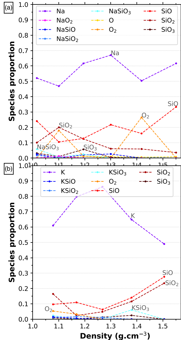
Figure 11. Proportion of all the isolated clusters of length less than 13 atoms as a function of density at 4000 K for (a) Na-feldspar and (b) K-feldspar end-members. Species that represent more than 5% of all the gas species for at least one density point are labeled in the graph. The other species, found in trace amounts, are the following (a) AlO, NaO, \text{Si}_2\text{O}_z ( z \in [3, 5] ) and some species among \text{Na}_w\text{Si}_x\text{O}_z ( w \in [1, 3] , x \in [1, 2] , z \in [1, 5] ); (b) O, \text{Si}_2\text{O}_3 , \text{Si}_2\text{O}_4 , \text{K}_w\text{AlO}_2 ( w \in [0, 1] ) and some species among \text{K}_w\text{Si}_x\text{O}_z ( w \in [1, 3] , x \in [1, 3] , z \in [3, 7] ).
