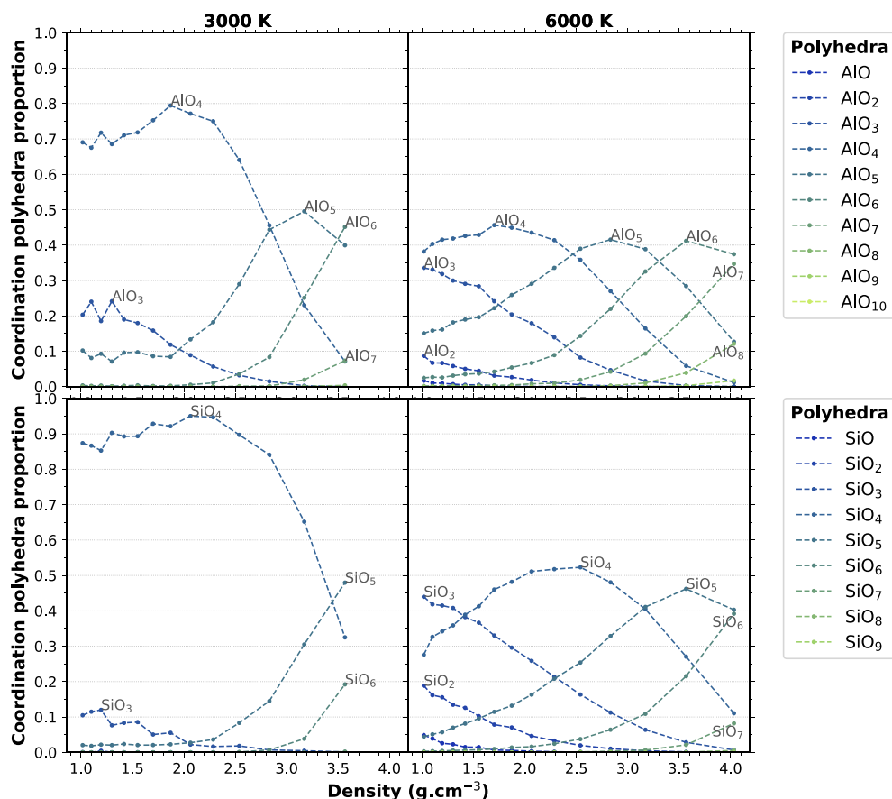
Figure 5. Relative proportion of \text{SiO}_x and \text{AlO}_x coordination species in \text{NaAlSi}_3\text{O}_8 for 3000 and 6000 K as a function of density.
