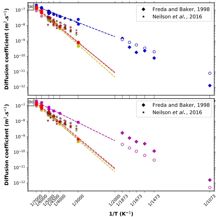
Figure 13. Self-diffusion coefficients for (a) Na-feldspar and (b) K-feldspar end-members at 1 GPa as a function of the inverse temperature (filled circles), and fit of the Arrhenius law (dashed lines). Colors indicate elements: red = O, yellow = Si, pink = Al, blue = Na, and purple = K. The stars indicate results from a classical MD simulation on molten albite (Neilson et al., 2016), and diamonds are experimental results on albite-orthoclase melts (Freda & Baker, 1998). Empty circles are the extrapolated diffusivities at the experimental temperatures using the Arrhenius fit of our data.
