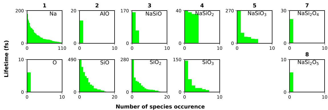
Figure 10. Lifetimes of isolated atomic clusters with less than 13 atoms at 1.02 \text{ g cm}^{-3} and 4000 K.
