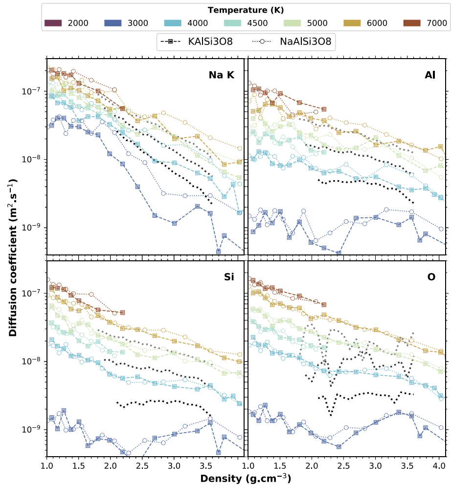
Figure 12. Self-diffusion coefficients for every element as a function of density. The black to light gray lines are theoretical results from Neilson et al. (2016) on \text{NaAlSi}_3\text{O}_8 at approximately 3000, 4000, and 5000K.
