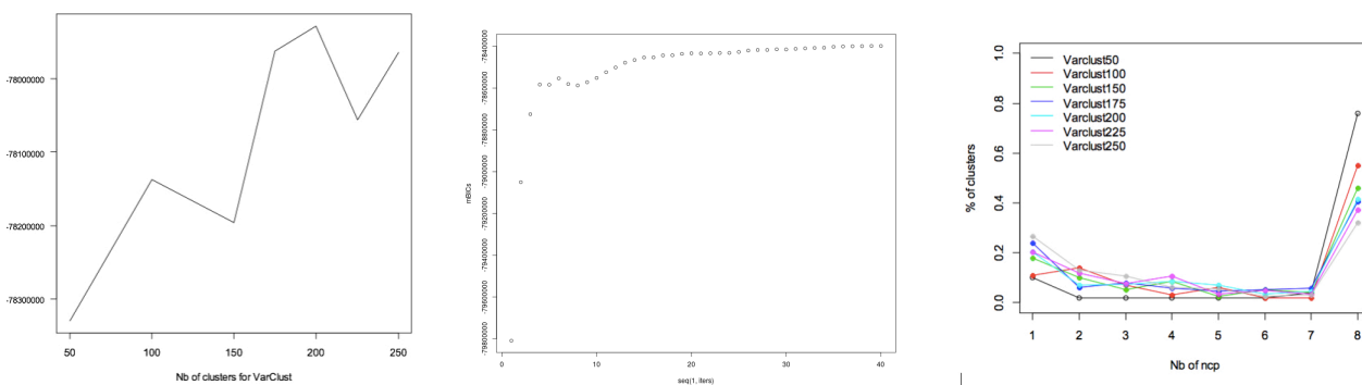
Figure 11: Left: evolution of the mBIC with the number of clusters; middle: evolution of the mBIC with the number of iterations; right: number of principal components in clusters in terms of K .
