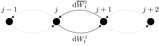
Figure 1. Representation of the lattice and the hopping amplitudes. A fermionic particle can jump to the right (resp. to the left) with probability per unit time dW_t (resp. d\bar{W}_t ). These amplitudes correspond to an effective interaction with a bosonic bath.
