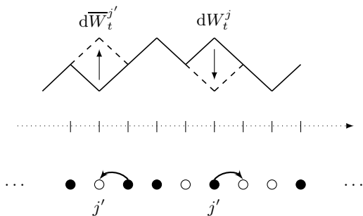
Figure 2. Classical mapping from the particle picture to the height field. Bottom. The particles can hop on the lattice, the occupied sites are black-filled and the rest is empty. Top. The configuration of particles can be represented by an interface incremented with the presence of a particle at the corresponding site. The particle transport maps to a corner growth process: if a particle hops to the left (resp. to the right) then a corner is raised (resp. lowered).
