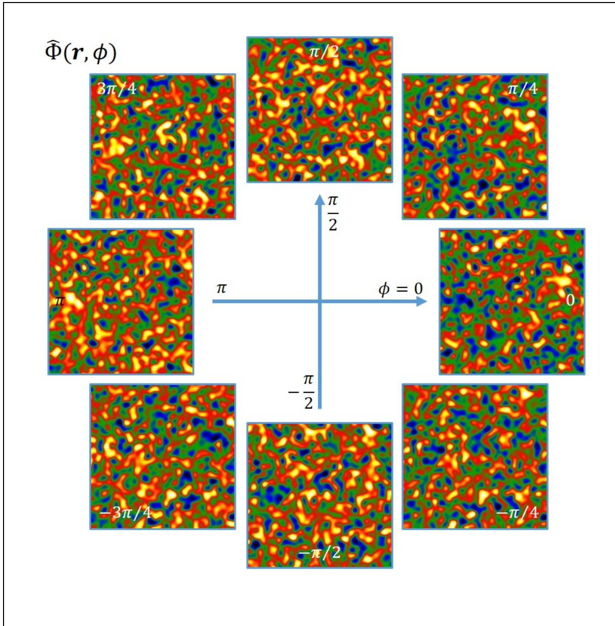
Figure 4. Phase noise from 5% gain variation as a function of initial phase, \phi : theoretical relative phase \hat{\Phi}(\mathbf{r}, \phi) calculated using Eq. (32). Colour range: \pm 50 mrad black to white.
