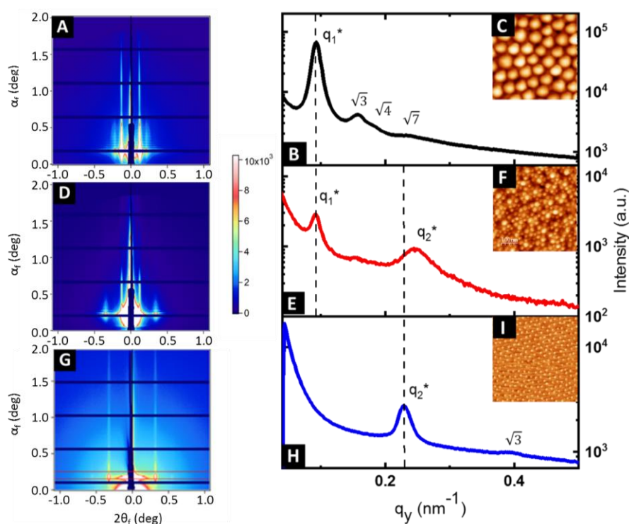
Figure 4. GISAXS patterns of (A) the \text{Al}_2\text{O}_3 dots formed by the infiltration of BCP1, (D) the bimetallic raspberry-like nanoclusters obtained by the combination of the small \text{Au}^0 NPs ( \sim 15 \text{ nm} diameter) on top of the \text{Al}_2\text{O}_3 dots ( \sim 36 \text{ nm} diameter) and (G) \text{Au}^0 NPs obtained using a nanostructured BCP2 film as a template. (B), (E) and (H) correspond to the GISAXS line-cuts along q_y integrated around the Yoneda band (Insets: AFM topographical images of the corresponding nanostructures).
