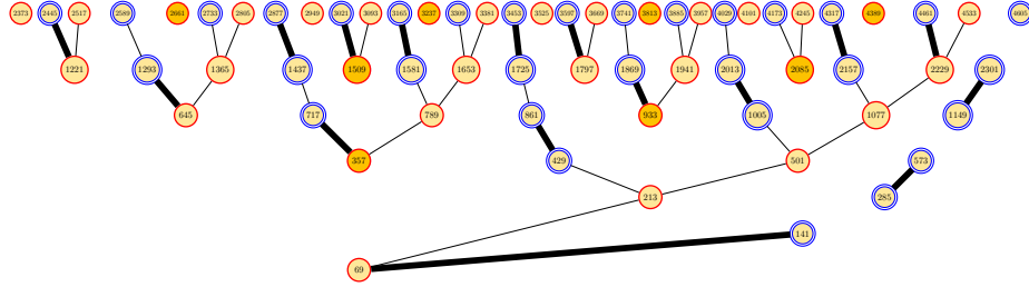
Figure 6. Representation of a Syracuse Determinant mapped onto a 2-4 Romanesco, made of the Triple A numbers that can be written V(a) where a is of type A. Each number is associated with a single integer, circled in blue if even, and red if odd. For any integer n , its associated Triple A is equal to 72n - 3 . The solid black lines plot the projection of the quaternary equivalence onto this representation. Only a subset of the Triple A numbers that are "vertical red" in this referential (i.e. that admit, in this representation, a V^{-1} that is itself a Triple A of odd integer n ; they are displayed in darker gold and they are +576 apart from each other in nominal value e.g. 357 + 576 = 933 ) actually needs to be solved to solve the Syracuse problem and that the Golden Automaton solves an infinity of Triple A numbers in a density that is sufficient to interdict the existence of any other independent "silver quiver" solves the Syracuse Problem.
