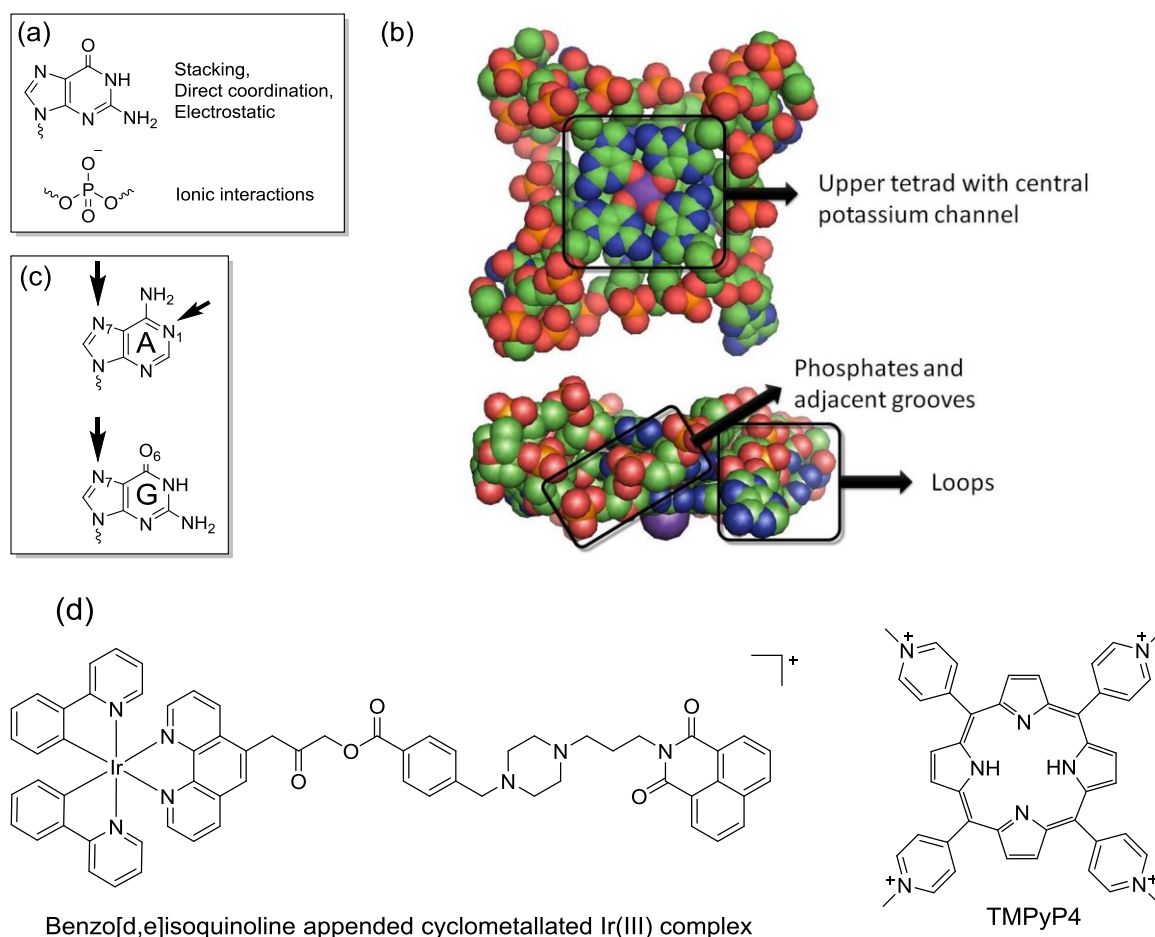
Figure 4. Main sites of interaction: (a) local sites; (b) global sites exemplified on the structure of the parallel human telomere quadruplex (pdb entry 1KF1); (c) Main platination sites; (d) Structure of compounds that interact through groove binding and/or stacking (see the text)
