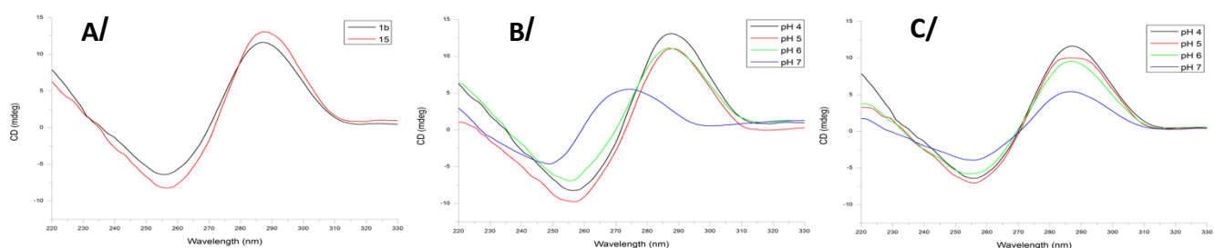
Figure 4. A/ CD spectra of biomolecular assembly 1b (black line) and control sequence 15 (red line) at pH = 4; B/ CD spectra of native telomeric sequence 15 at different pH; C/ CD spectra of biomolecular assembly 1b at different pH. Measurements were carried out at 2 \mu M in 10 mM PBS buffer at 20°C.
