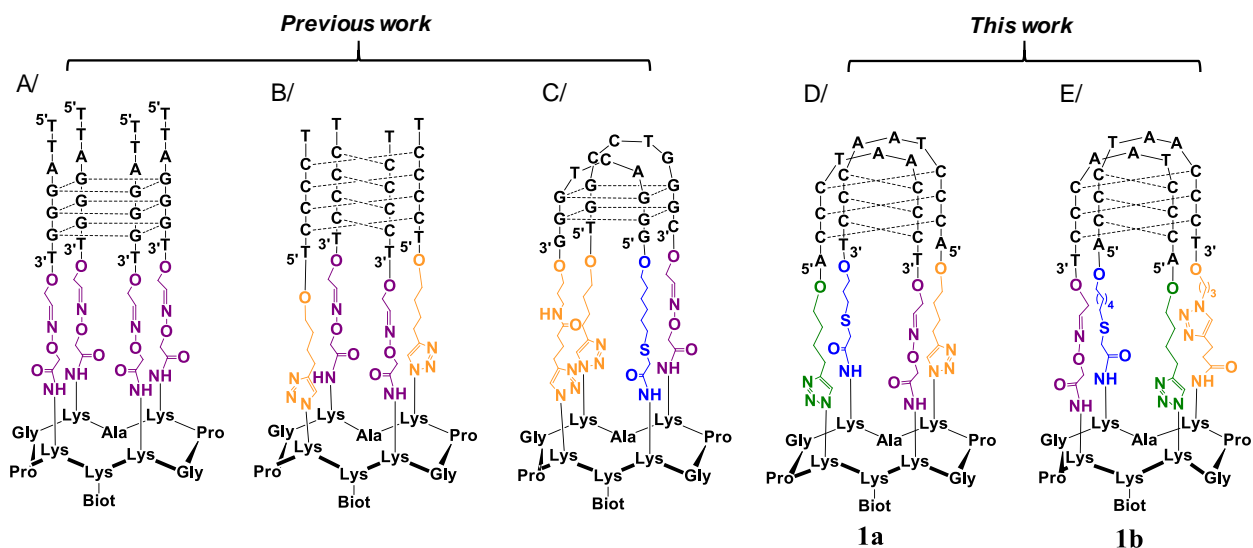
Figure 2. Use of cyclopeptide scaffold for the design of stabilized tetraplex DNA structures: A/ Parallel G4-DNA, 19a B/ I-motif DNA structure without loops, 22 C/ Antiparallel G4 structure from HIV virus sequence, 23 D/ Telomeric i -motif mimic 1a and E/ Telomeric i -motif mimic 1b . For the sake of clarity, the positive charges shared by the two cytosines involved in the C-C base pairs of structures B, D and E are not displayed. Dotted lines represent the base pairing.
