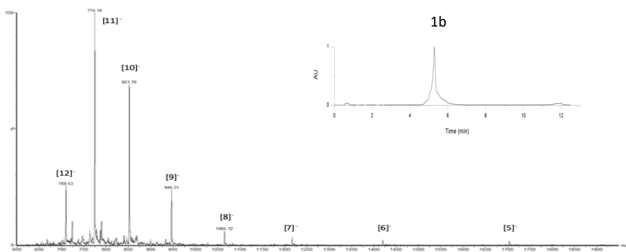
Figure 3. UPLC-MS monitoring of OL for the crude transformation of 14 to 1b corresponding to all peak. Insert: UPLC profile of crude mixture, column heated at 60°C, detection at 260 nm.
