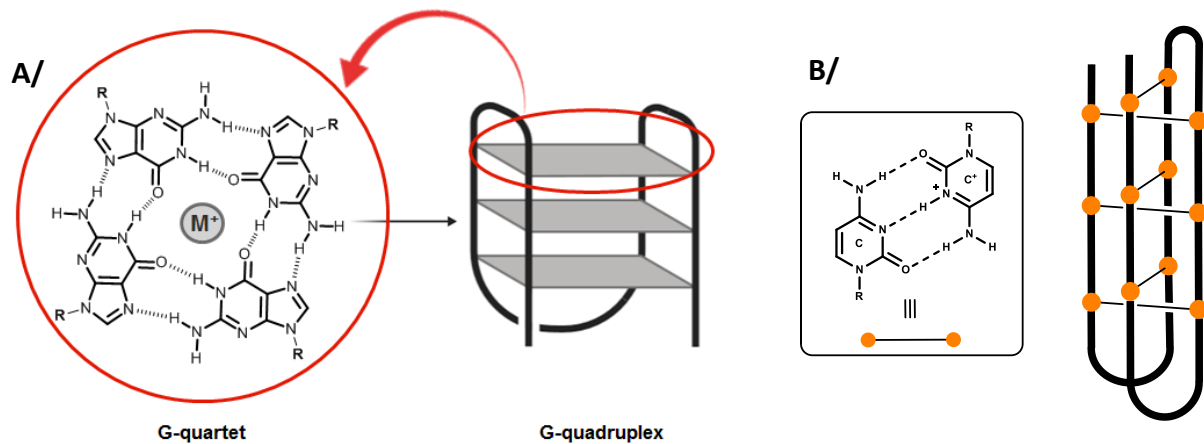
Figure 1. A/ G-quartet with Hoogsteen hydrogen bonded guanine and schematic drawing of a G4 structure and B/ hemi-protonated C-C+ base pairs and schematic representation of an i -motif structure.
