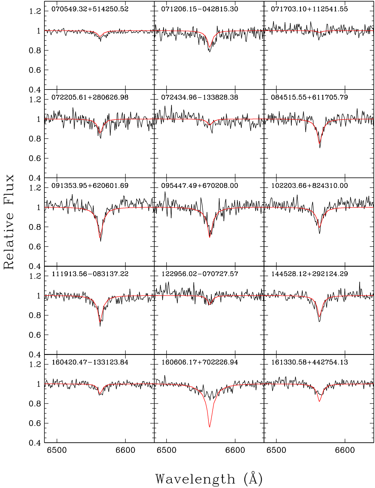
Figure A9. Comparison of observed and predicted H \alpha line profiles from Gaia photometric parameters (continued 2/4).
