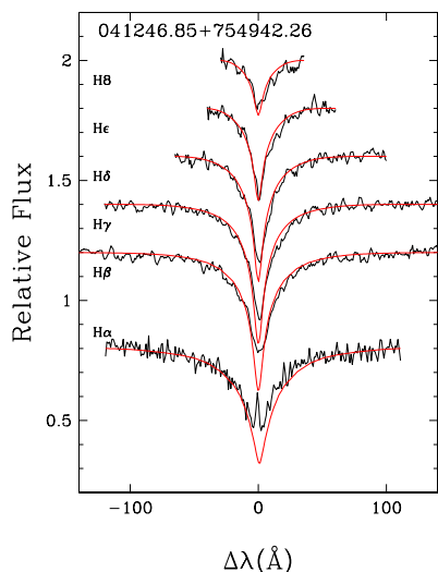
Figure 4. Comparison of the normalised observed Balmer line profiles for WD J0412+7549 with a DA model atmosphere at the Gaia derived photometric parameters ( T_{\text{eff}} = 8510 K and \log g = 8.25 ). Lines are offset vertically for clarity.
