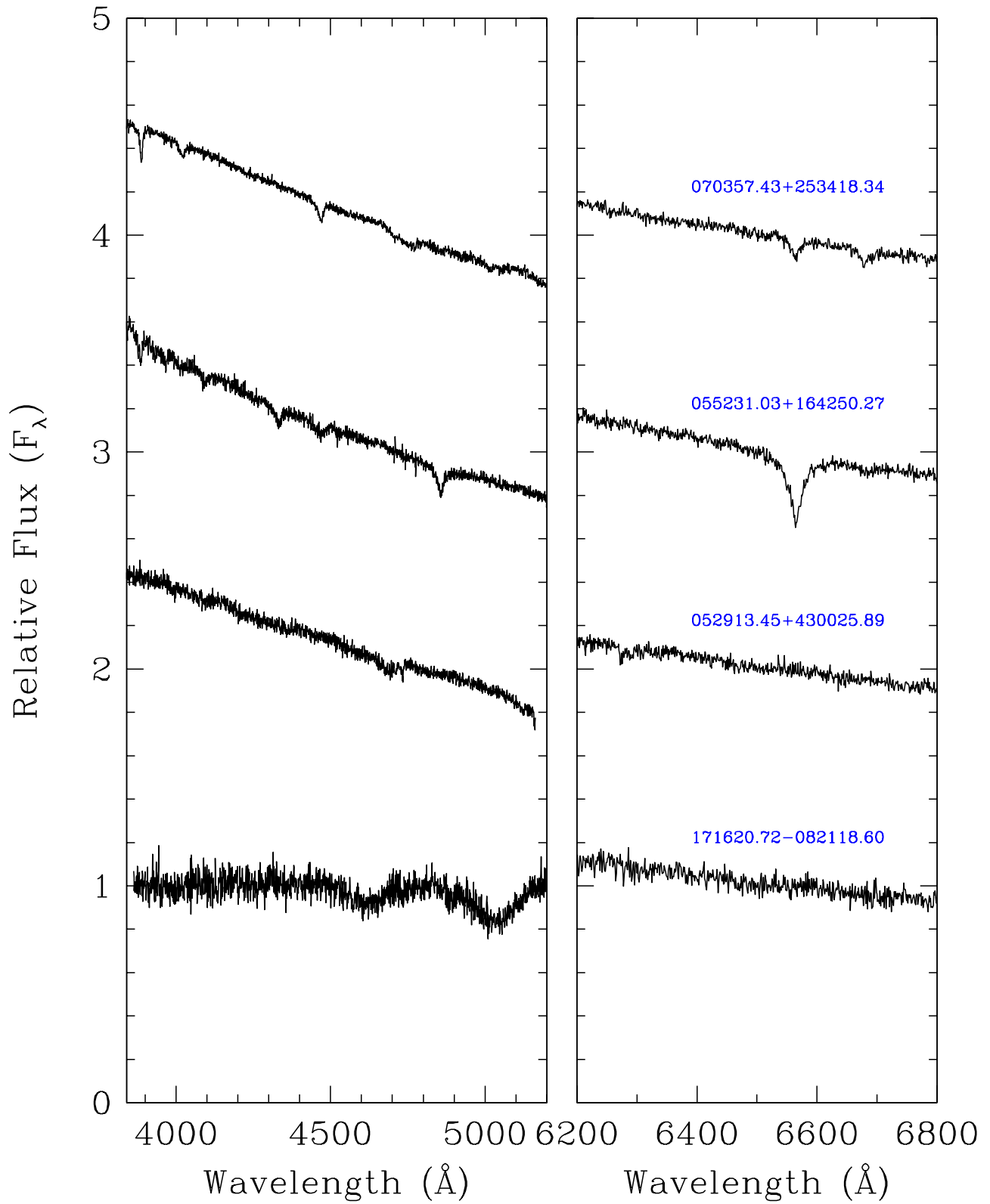
Figure A13. Spectroscopic observations of two DBA (top) and two DQ white dwarfs (bottom).
