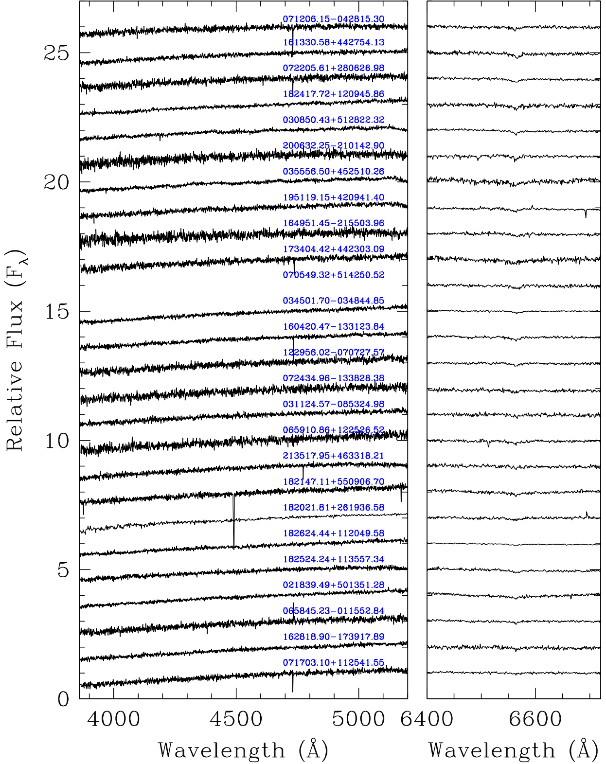
Figure A4. Spectroscopic observations of 89 DA white dwarfs ordered with decreasing photometric temperature (continued 4/4).
