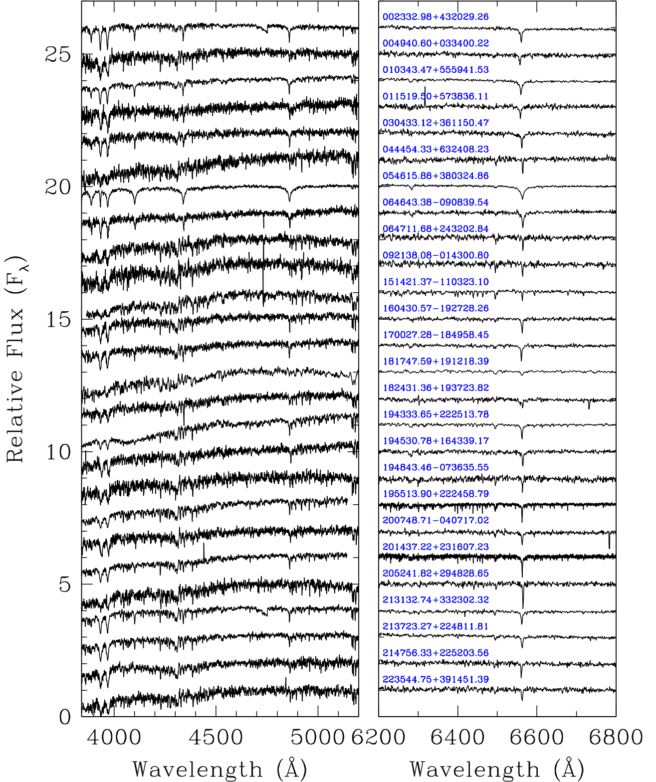
Figure A20. Spectroscopic observations of main-sequence stars that are low-probability white dwarf candidates ( P_{\text{WD}} < 0.75 ) in the catalogue of Gentile Fusillo et al. (2019).
