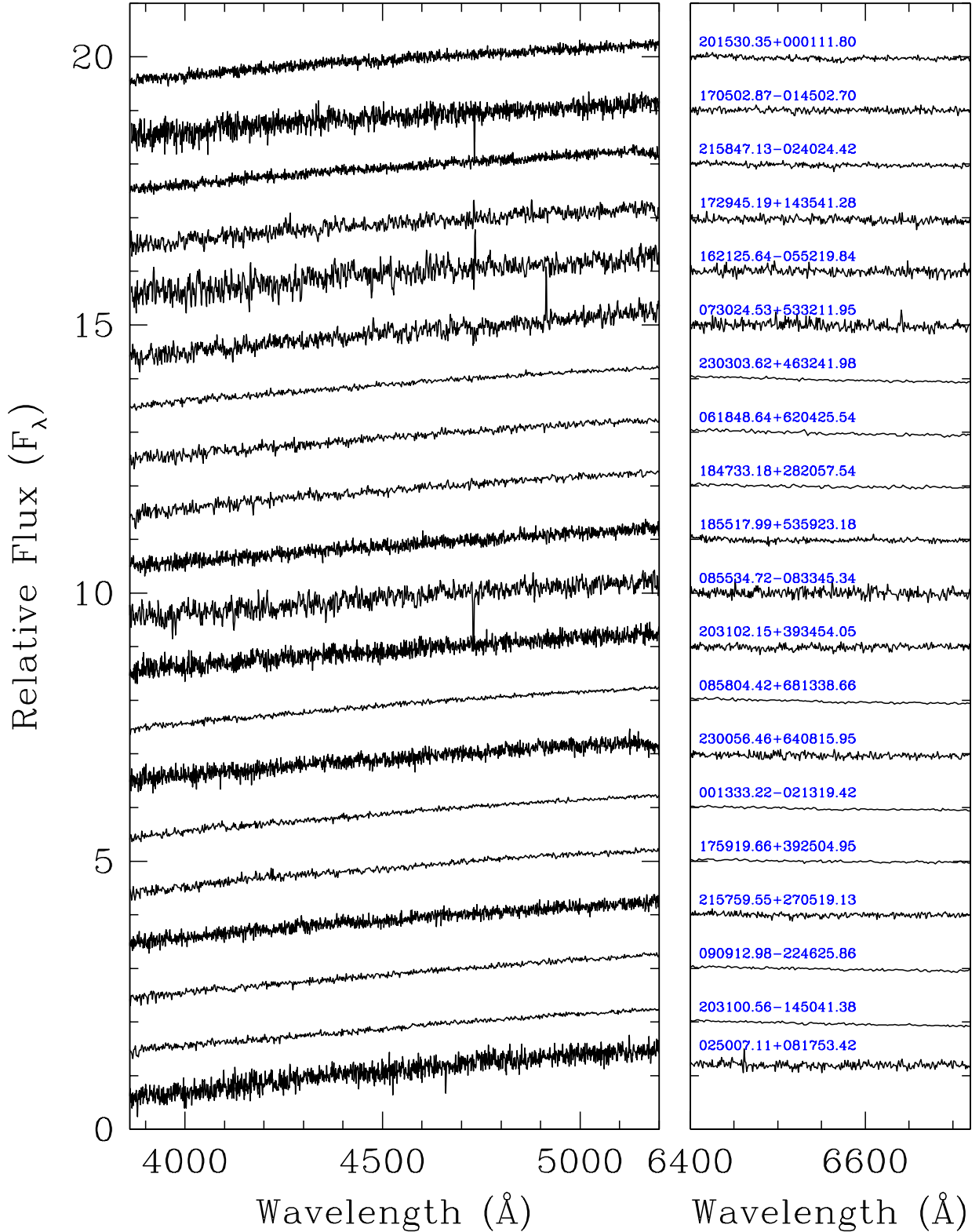
Figure A16. Spectroscopic observations of 76 DC white dwarfs ordered with decreasing photometric temperature (continued 3/4).
