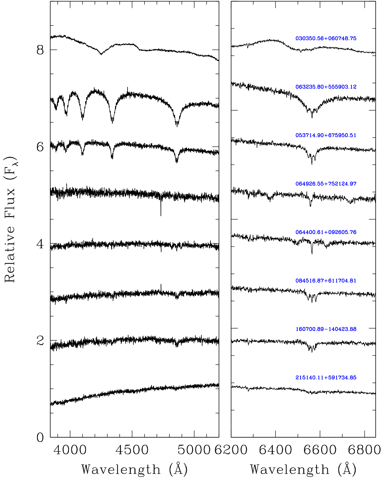
Figure A12. Spectroscopic observations of eight magnetic white dwarfs ordered with decreasing temperature and excluding the DZH WD J1515+8230, shown instead on Fig. A18.
