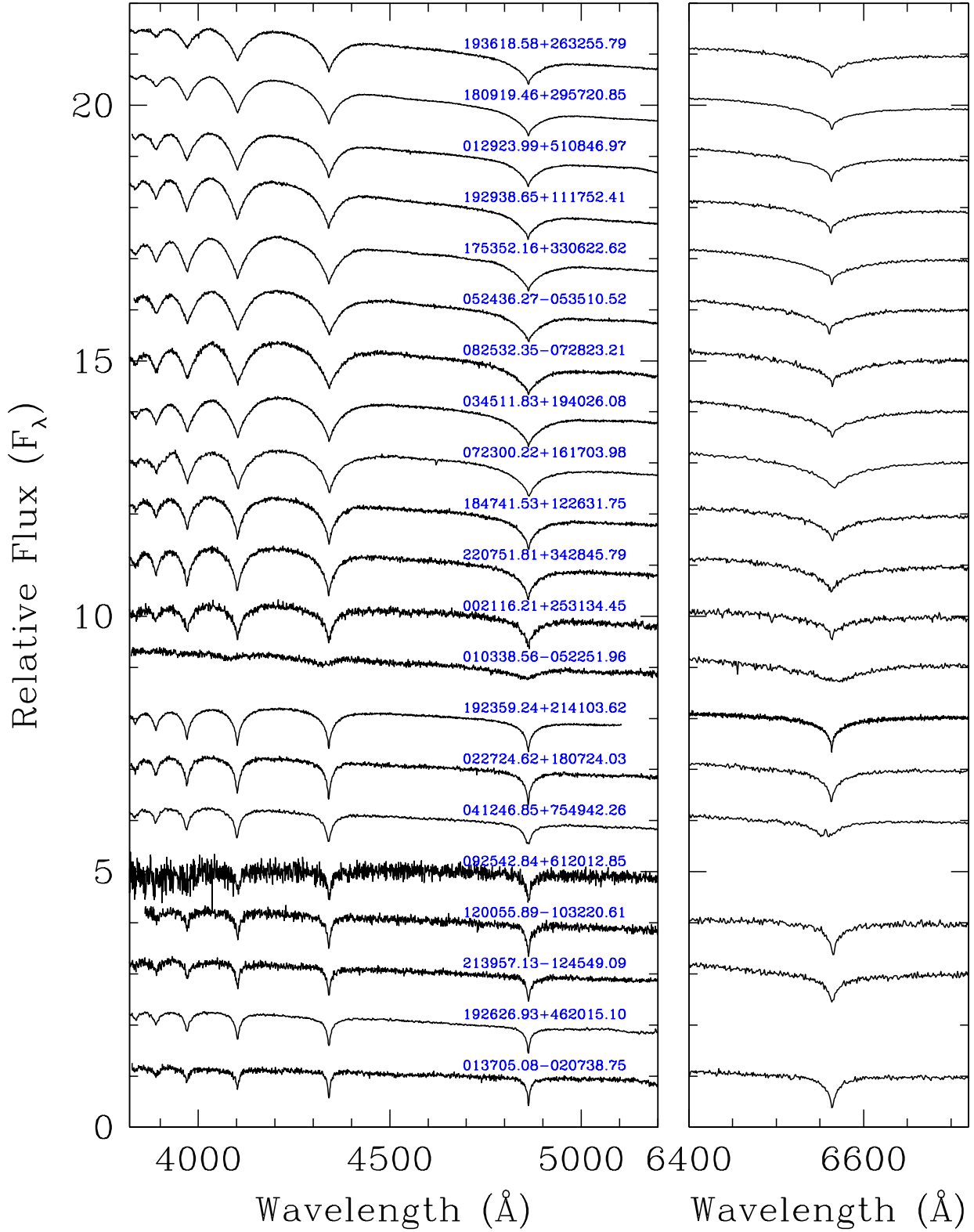
Figure A1. Spectroscopic observations of 89 DA white dwarfs ordered with decreasing photometric temperature (continued on Figs. A2-A4).
