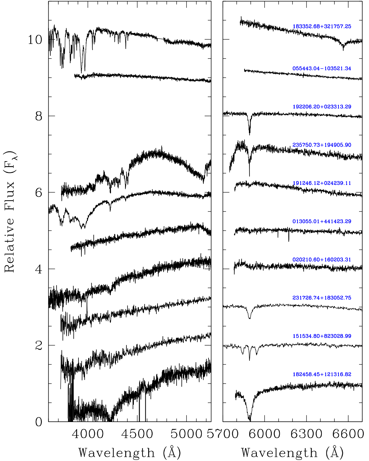
Figure A18. Spectroscopic observations of 10 DZ, DZA and DZH white dwarfs.
