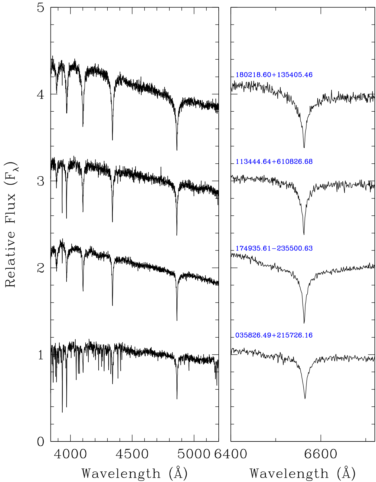
Figure A5. Spectroscopic observations of 4 DAZ white dwarfs ordered with decreasing photometric temperature.
