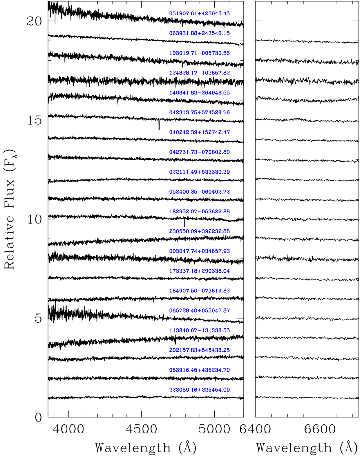
Figure A14. Spectroscopic observations of 76 DC white dwarfs ordered with decreasing photometric temperature (continued on Figs. A15-A17).
