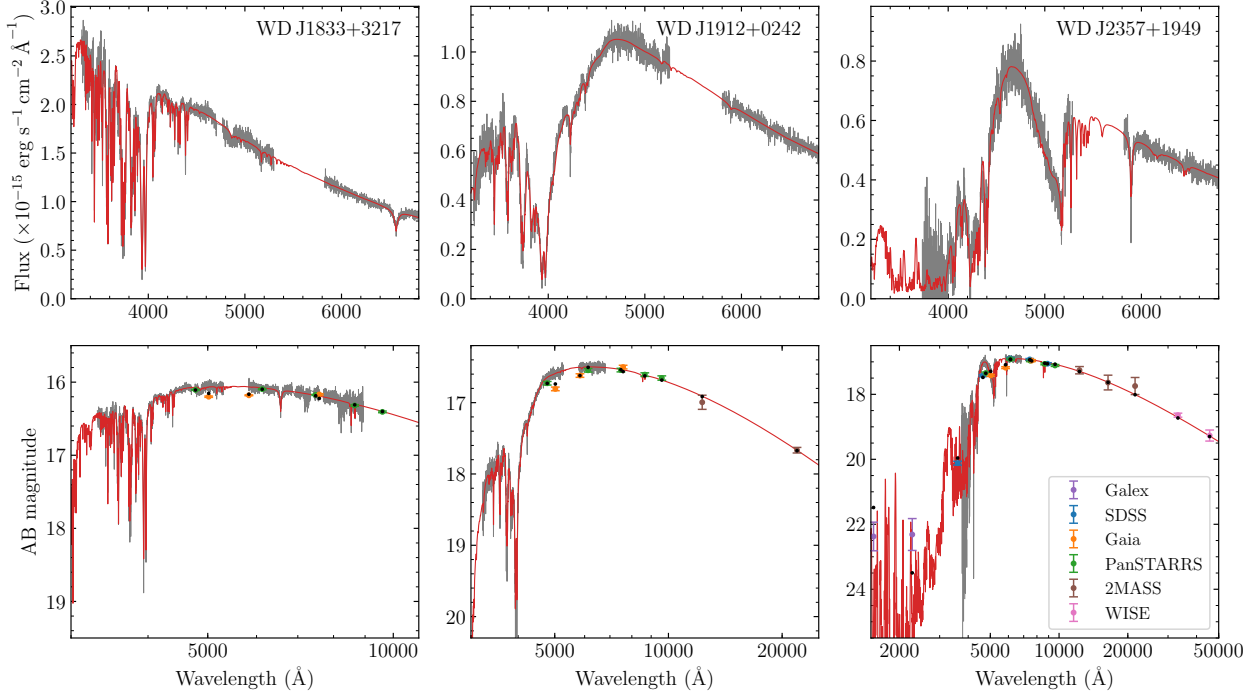
Figure 5. Simultaneous fits of spectroscopy and photometry for the DZA 183352.68+321757.25 (left panels), DZ 191246.12+024239.11 (middle panels) and DZ 235750.73+194905.90 (right panels). The top row of panels compare our best fit models to normalised spectroscopic observations. The spectroscopic observations are recalibrated onto the models to deal with flux-calibration quirks, but are still in physical flux units. The bottom panels compare our best fit models to catalogue photometry over a wider wavelength range. All three objects have helium-dominated atmospheres and fit parameters are given in Table 6. For WD J1912+0242, the K -band is from UKIDSS rather than 2MASS.
