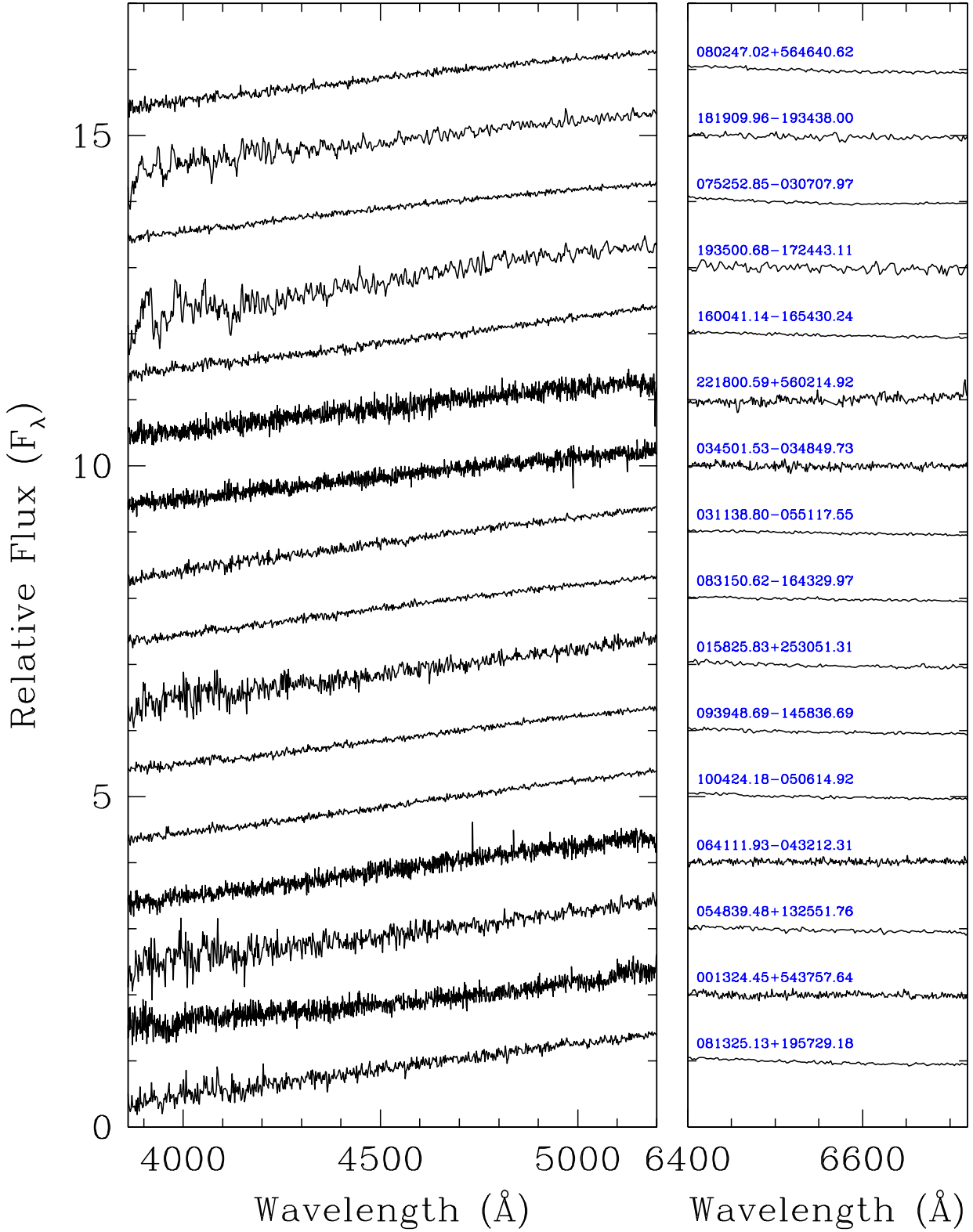
Figure A17. Spectroscopic observations of 76 DC white dwarfs ordered with decreasing photometric temperature (continued 4/4).
