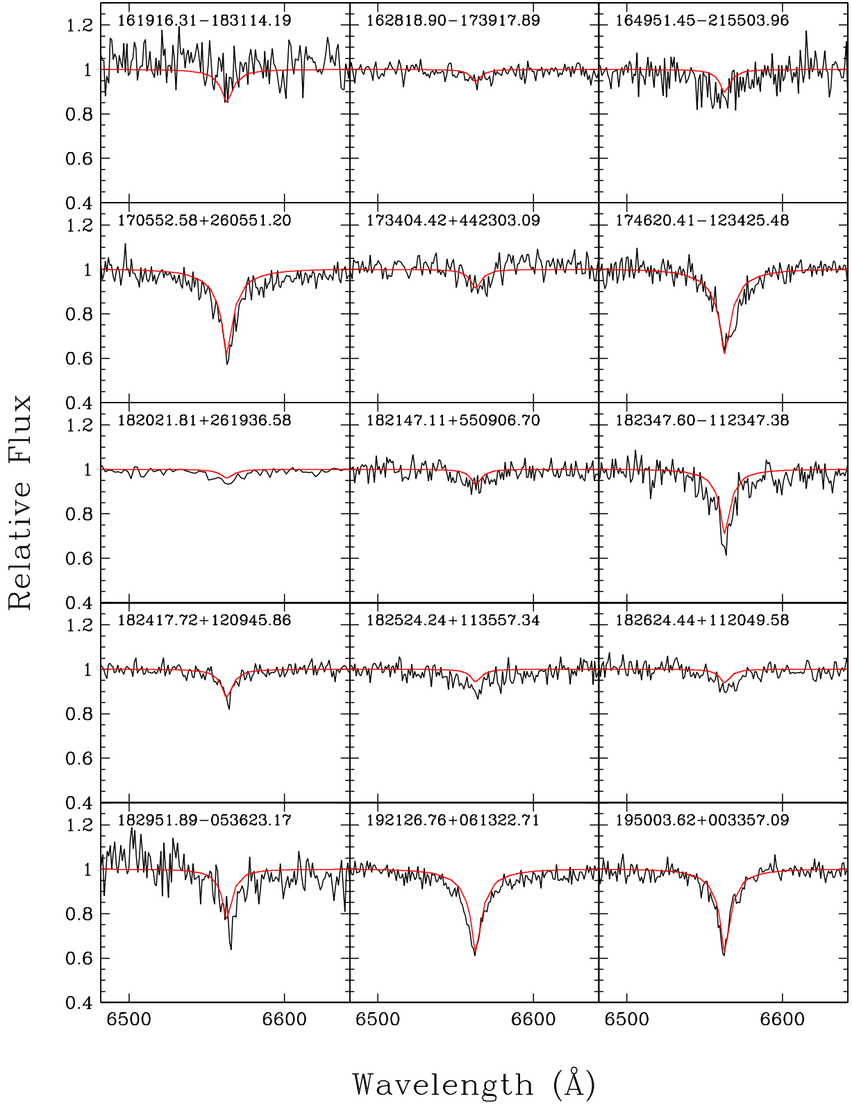
Figure A10. Comparison of observed and predicted H \alpha line profiles from Gaia photometric parameters (continued 3/4).
