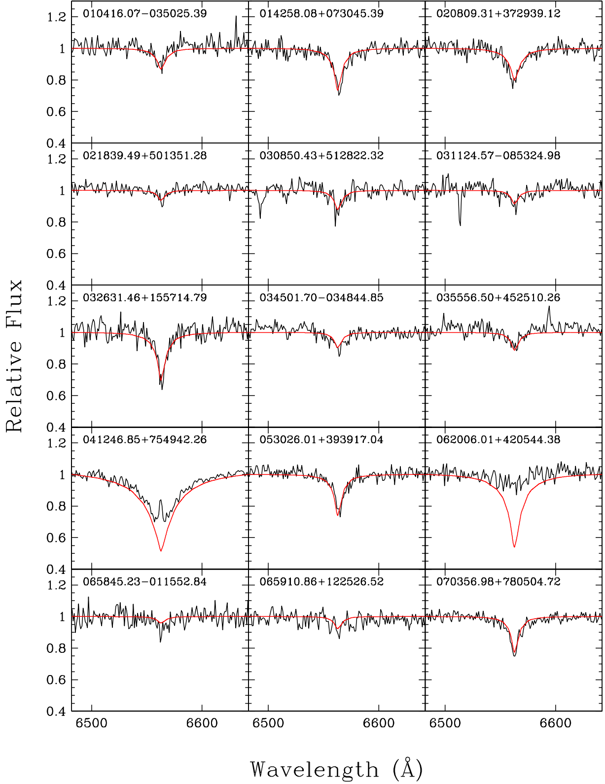
Figure A8. Comparison of observed and predicted H \alpha line profiles from Gaia photometric parameters. 51 DA stars are shown, including all of those with Gaia parameters below 6000 K in addition to the DAe WD J0412+75494 and He-rich DA WD J0620+4205 and WD J1606+7022. A correction of +2.7% to the Gaia temperatures was applied. Continued on Figs. A9-A11.
