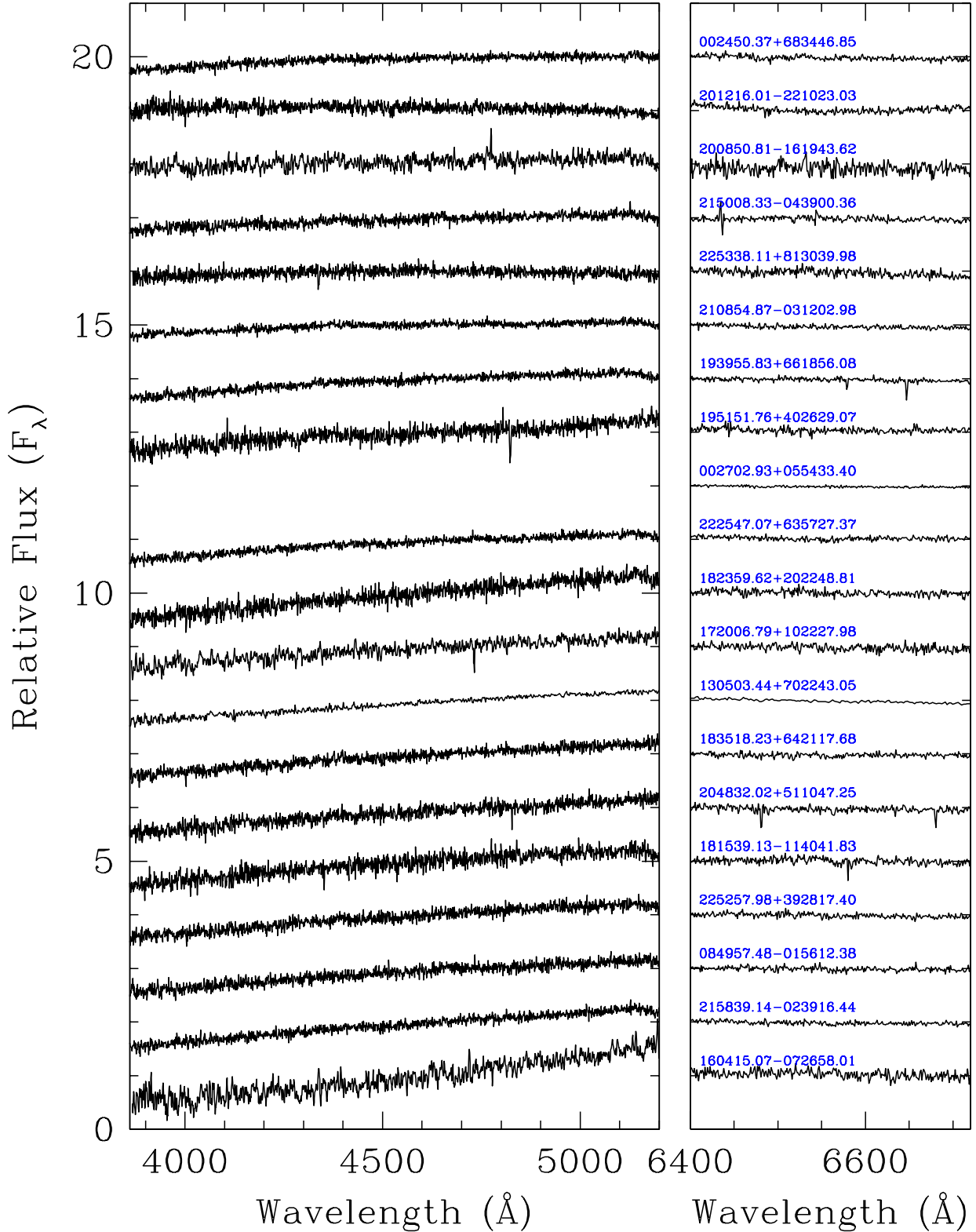
Figure A15. Spectroscopic observations of 76 DC white dwarfs ordered with decreasing photometric temperature (continued 2/4).
