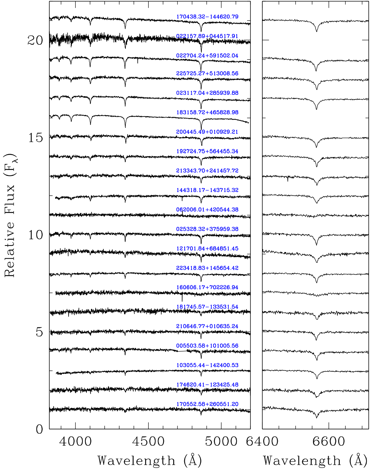
Figure A2. Spectroscopic observations of 89 DA white dwarfs ordered with decreasing photometric temperature (continued 2/4).
