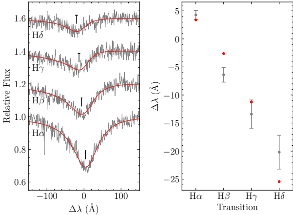
Figure 3. Left: Asymmetric-Lorentzian profile fits to H\alpha – H\delta for WD J0103–0522. The black T symbols mark the position of the best fit to the profile minimum, with their widths indicating the 1\sigma uncertainties. Right: The measured values of the profile minima, fitted with a redshift of 261 \pm 40 \text{ km s}^{-1} , and field strength of 4.8 \pm 0.4 \text{ MG} (red points).
