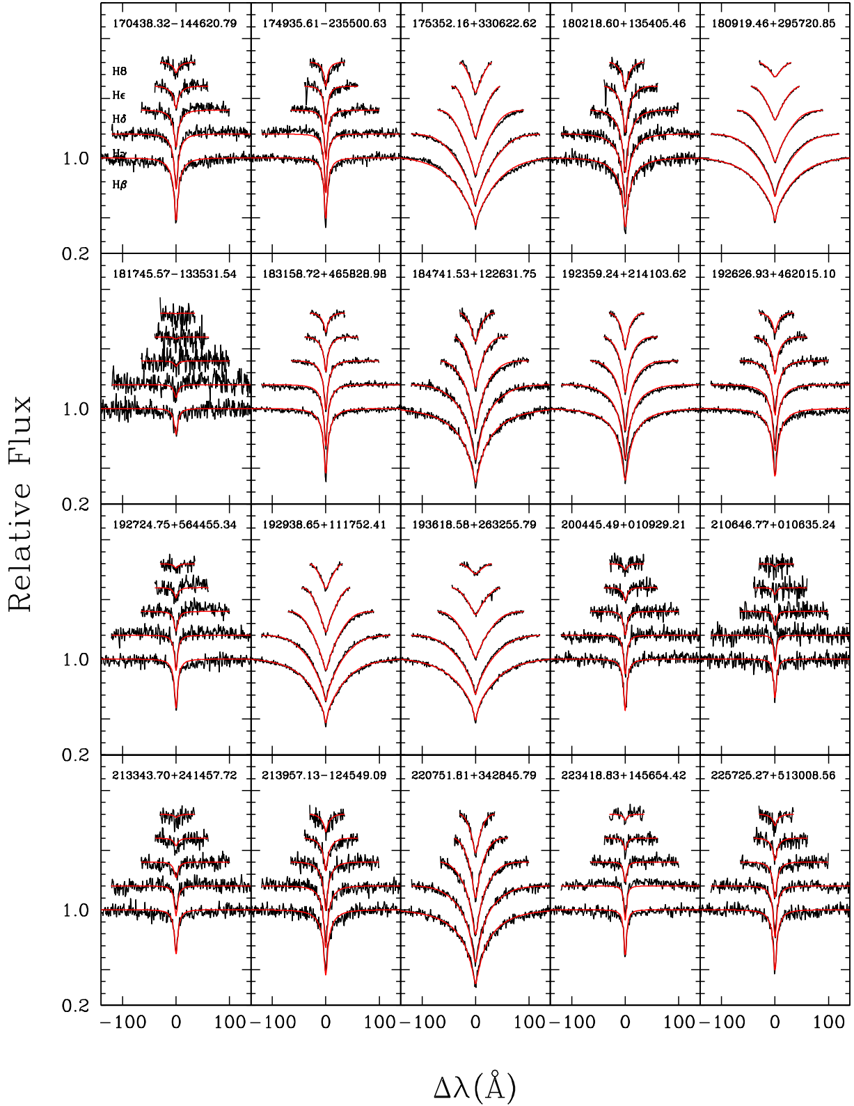
Figure A7. Fits to the normalised Balmer lines for 40 DA and DAZ white dwarfs (continued 2/2).
