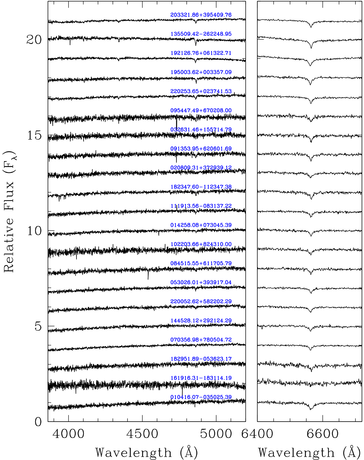
Figure A3. Spectroscopic observations of 89 DA white dwarfs ordered with decreasing photometric temperature (continued 3/4).
