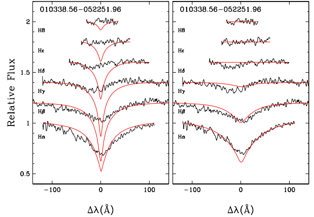
Figure 2. (Left:) Comparison of the normalised observed Balmer line profiles for WD J0103–0522 with a DA model atmosphere at the Gaia derived photometric parameters ( T_{\text{eff}} = 8960 K and \log g = 9.34 ). (Right:) Fit of the observations using He-rich model atmospheres with [\text{H}/\text{He}] = -1.70 . The resulting best fit parameters ( T_{\text{eff}} = 8520 K and \log g = 9.06 ), excluding the constraint from parallax, should be taken with caution given the relatively poor quality of the fit and we consider the photometric parameters more reliable.
