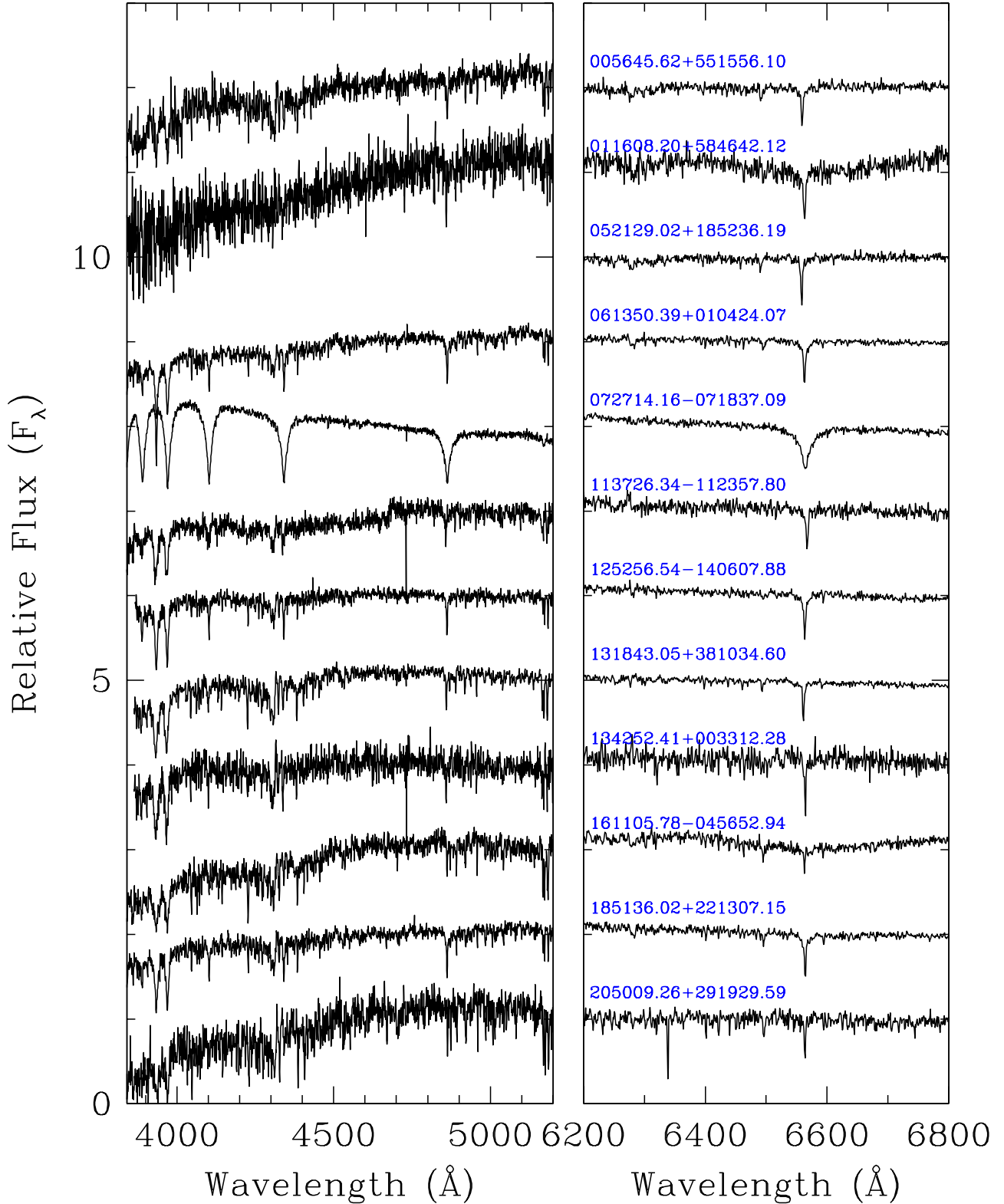
Figure A19. Spectroscopic observations of main-sequence stars that are high-probability white dwarf candidates ( P_{\text{WD}} > 0.75 ) in the catalogue of Gentile Fusillo et al. (2019).
