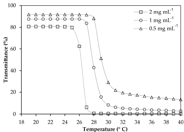
Figure 9. Effect of the concentration on the LCST of the PNVL- b -PCL (1) block copolymer micelles.
