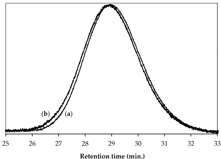
Figure 1. Size exclusion chromatography (SEC) chromatogram of PNVCL homopolymer before (a, X-PNVCL-OH) and after (b, PNVCL-OH) chain end removal by reaction with 2,2'-azobis(isobutyronitrile) (AIBN).
