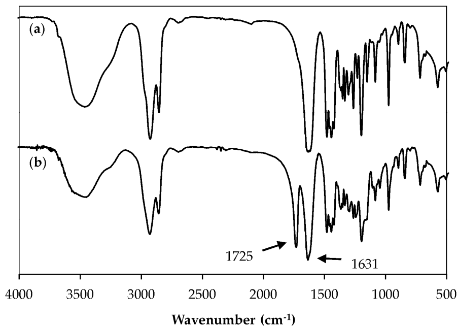
Figure 5. FTIR spectra of (a) PNVCL-OH and (b) PNVCL- b -PCL (1).
