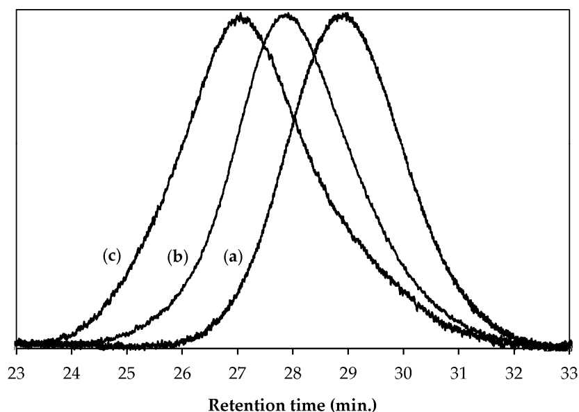
Figure 4. SEC chromatograms of (a) PNVCL–OH, (b) PNVCL- b -PCL (1) and (c) PNVCL- b -PCL (2).
