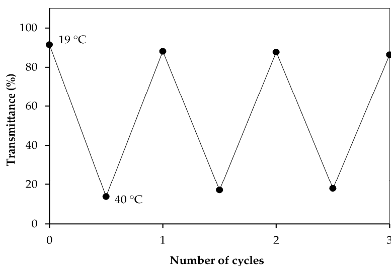
Figure 12. Transmittance cycling of the PNVCL- b -PCL (1) block copolymer micelle solution ( 0.5 \text{ mg mL}^{-1} ) between 19 and 40 \text{ }^{\circ}\text{C} .
