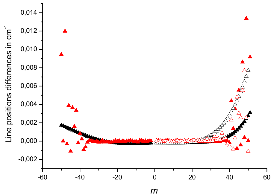
Fig. 11. Line positions differences plotted versus m ( m = -J, J, J+1 for P, Q, R branch respectively) for the 00001\ 0\ 1 - 00000\ 0\ 0 band ( \nu_3^1 ). (HITRAN – Calculation (this work)) and (HITRAN – EXOMOL) are plotted in black and red symbols respectively. Solid up-triangles correspond to P_{ee} and R_{ee} -branches, open up-triangles for Q_{ie} -branch.
