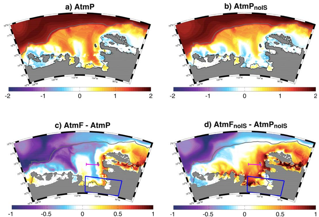
Figure 3. Conservative ocean temperature ( ^{\circ}\text{C} ) averaged over 200–1,000 m (annual mean over the 13th simulation year) in (a) AtmP and (b) AtmP noIS . Wind-induced ocean temperature anomalies defined as (c) AtmF minus AtmP and (d) AtmF noIS minus AtmP noIS . The magenta line ( 73^{\circ}\text{S} 105^{\circ}\text{W} 109^{\circ}\text{W} ) is across the Pine Island Trough and is used to calculate horizontal transports in Figure 9. The blue box ( 76^{\circ}\text{S} 74.3^{\circ}\text{S} 96^{\circ}\text{W} 109^{\circ}\text{W} ) is used throughout the paper to average vertical transport, temperatures, and heat budget terms near the fronts of Pine Island and Thwaites glaciers. The grey line represents the continental shelf break (1,500 m isobath).
